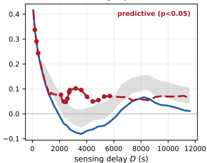
GOES X-ray · space wx
