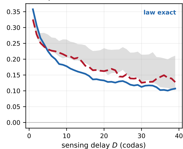
Sperm-whale codas · bioacoustics
