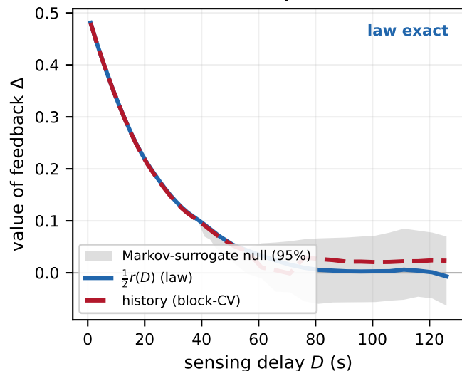
Two-state Markov (synth) · reference
