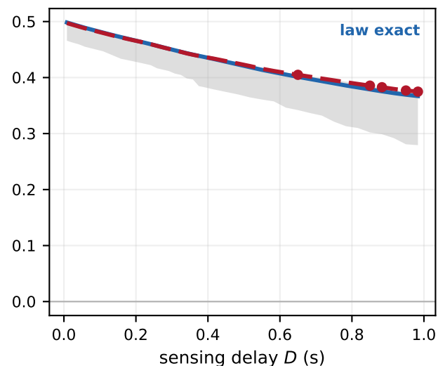
LOCATA azimuth · acoustics
