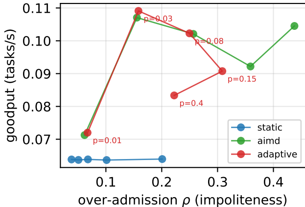
Goodput-politeness Pareto
