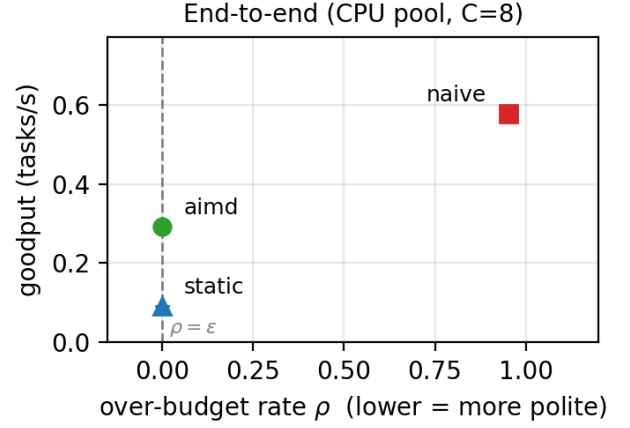
Fig. 5. Goodput vs. over-budget \rho , CPU pool ( C=8 ). With surplus capacity the separation widens: aimd delivers 3.18 \times static's goodput at \rho = 0 , while naive buys goodput only by flagrant over-admission ( \rho = 0.95 ).
