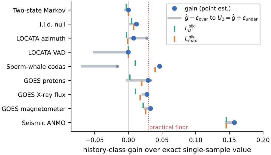
Fig. 3. The battery at a glance. Dots: maximum history-class gain over the exact single-sample value; grey bars: the model-calibrated interval [\hat{g} - \epsilon_{\text{over}}, \hat{g} + \epsilon_{\text{under}}] ; ticks: the moving-block one-sided bounds at fixed D^* (upper, teal) and with in-replicate lag selection (lower, orange); dotted line: the registered practical floor. Only seismic separates decisively from both zero and the floor; the i.i.d. null's positive selection-aware tick is the empirical winner's-curse floor; whale's wide bar is the short-series noise the verdict language respects. Where \epsilon_{\text{under}} < 0 (whale, i.i.d.) the bias-corrected upper endpoint U_2 sits below the point estimate, because the estimator is upward-biased there, and the bound says so.
