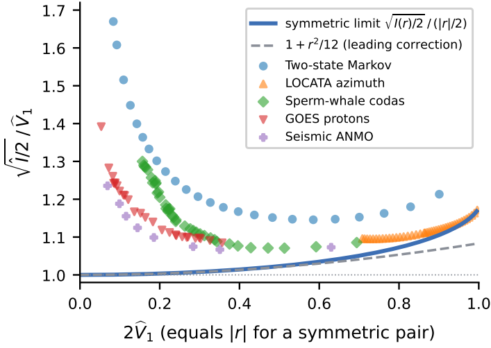
Fig. 2. Tightness of the information envelope on approximately balanced binary pairs (Proposition 3.5). Points: per-lag ratio \sqrt{\hat{I}/2} / \hat{V}_1 of the information envelope to the exact single-sample value, both computed from the same pooled lag table, for the series with |\hat{\pi} - \frac{1}{2}| < .035 (lags with \hat{V}_1 > .025 ; the i.i.d. null has none). Theorem 3.1 applied to that table forces every point to at least one. The horizontal axis is 2\hat{V}_1 , which equals |r| for a symmetric pair, so the curve is the symmetric limit \sqrt{I(r)/2} / (|r|/2) and the dashes its leading correction 1 + r^2/12 . Points above the curve at small \hat{V}_1 are the mildly imbalanced series, whose single-sample value is pulled toward Theorem 6.1's threshold (Fig. 1). A consistency check, not an independent test.
