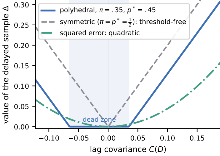
Fig. 1. The contact-order trichotomy (Theorem 6.3), drawn exactly. Polyhedral objective with \pi=.35 , one kink at p^*=.45 , \Delta s=2 : sign-dependent hinges with dead-zone thresholds a^+=.035 (positive branch) and a^-=.065 (negative branch), so anticorrelation of the same magnitude can be worthless where positive correlation has value. The symmetric case is the threshold-free degenerate hinge; squared error responds quadratically with no dead zone. The axis spans exactly the feasible covariance range [-\pi^2, \pi(1-\pi)] ; for stronger asymmetry (e.g. \pi=.2 , p^*=.3 ) the negative-branch threshold exceeds the feasible range entirely and anticorrelated sensing is worthless at every achievable covariance.
