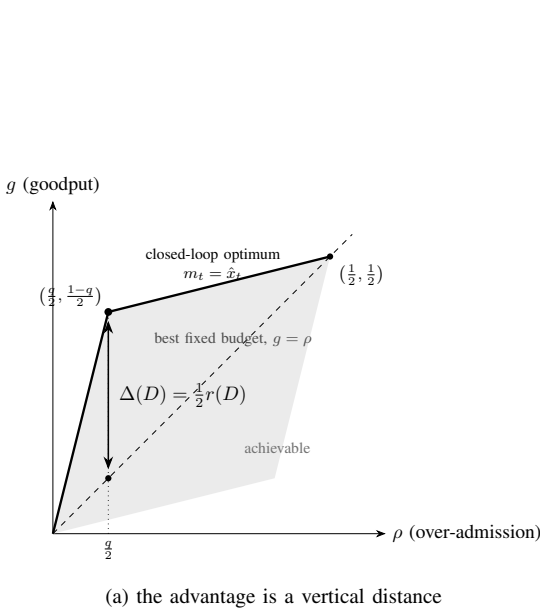
Fig. 2. (a) Under age- D sensing the achievable (\rho, g) pairs form the shaded hull. Fixed budgets lie on the diagonal g = \rho , and the closed-loop optimum sits a vertical \Delta(D) = \frac{1}{2}r(D) above it (Thm. 1). (b) The same value \frac{1}{2}e^{-D/\tau_c} over the sensing-age and coherence-time plane with \tau_c on a log scale. Points are the measured Markov contention sweep of Cor. 1, each shaded by the adaptive controller's closed-loop fraction, opening onto the fixed budget as D crosses \tau_c .
