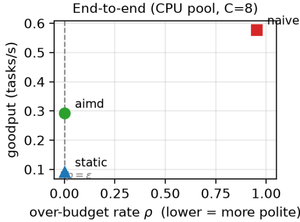
Fig. 3. Goodput vs. over-budget \rho , CPU pool ( C=8 ). With surplus capacity the separation widens: aimd delivers 3.18\times static’s goodput at \rho = 0 , while naive buys goodput only by flagrant over-admission ( \rho = 0.95 ).
