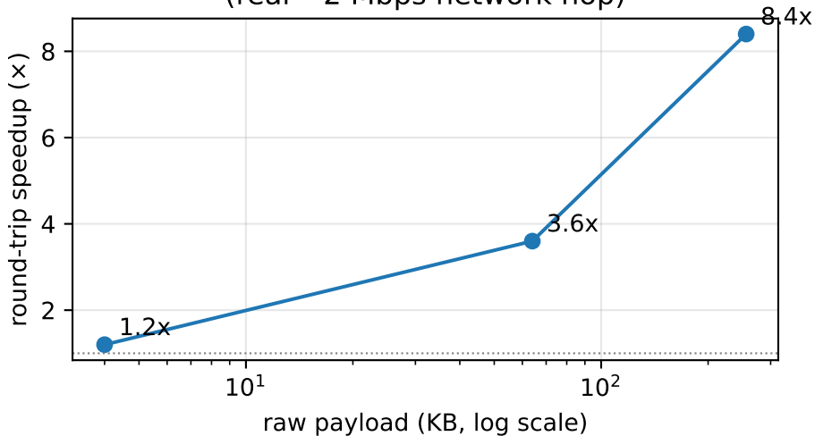
Tier 2: compression speedup vs payload (real ~2 Mbps network hop)
