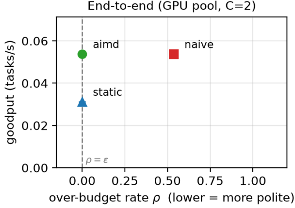
Fig. 2. Goodput vs. over-budget \rho , GPU pool ( C=2 ). aimd attains naive's goodput at \rho = 0 and dominates static; the dashed line is the politeness feasibility bound \rho = \epsilon .
