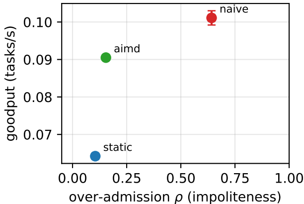
Contended Pareto (square)
