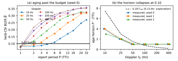
Fig. 3. The age horizon at the true 0.10 budget (calibrated baseline; pilot-2 shakedown, graded seeds swap in after the 2026-08-27 seal). (a) Held-CSI BLER against report period. (b) The horizon collapses to a few TTI at low mobility and the frame minimum above 50 Hz.
