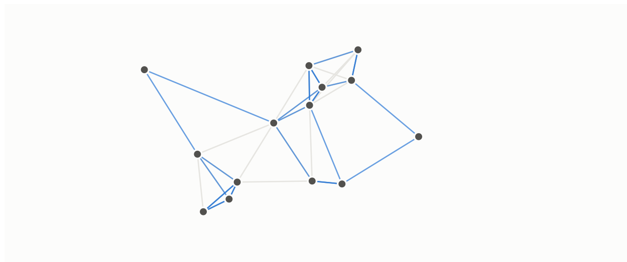
Figure 144: The row at minimal distance from a query.
