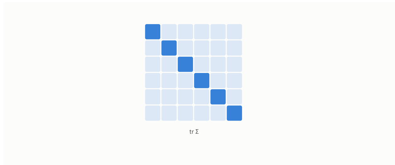
Figure 227: The sum of the diagonal, the total variance for a covariance.
