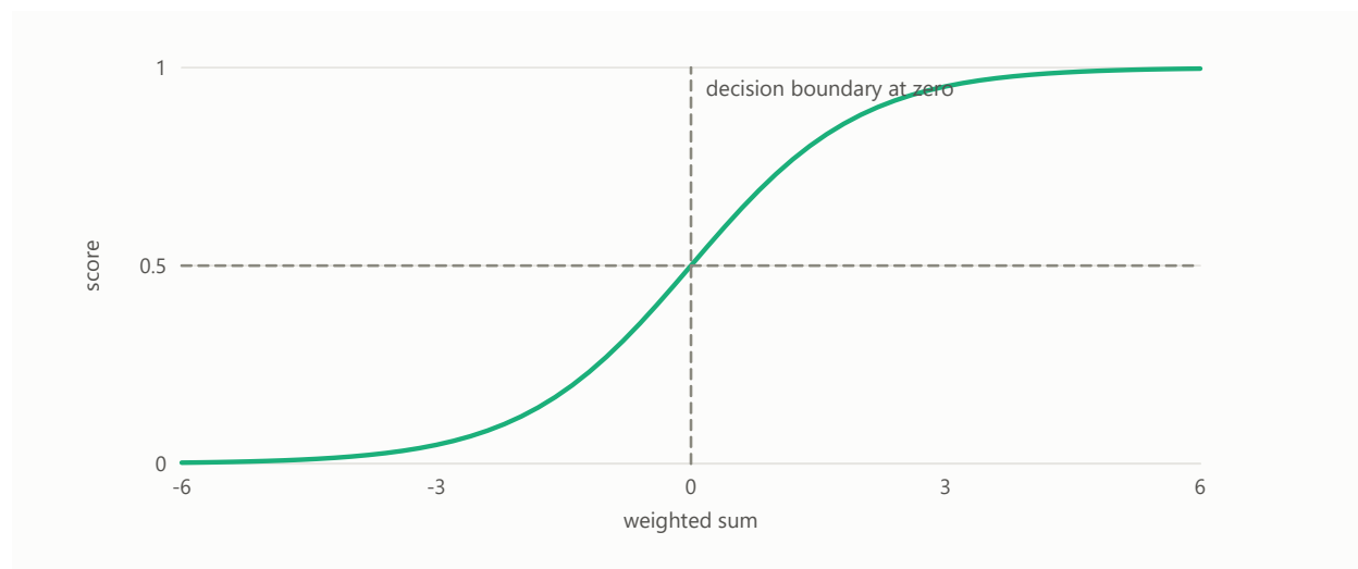
Figure 131: The sigmoid of a weighted sum, above one half on one side of the hyperplane.
