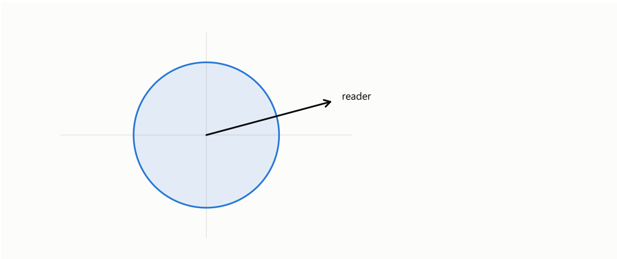
Figure 97: The normal distribution, isotropic when every direction is the same.
