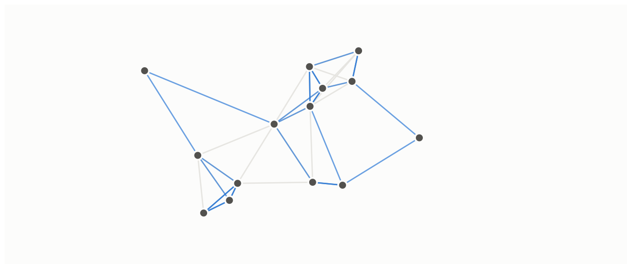
Figure 99: Nodes and the edges that join pairs of them.
