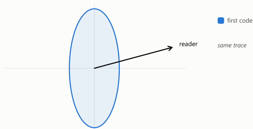
Figure 146: The directions the consumer never reads, the kernel of its read operator.
