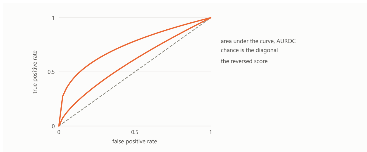
Figure 138: Optimal thresholded F1 survives any strictly monotone transform, AUROC only an increasing one.
