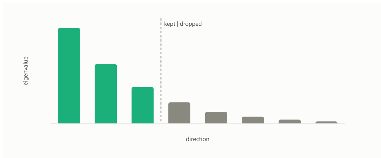
Figure 230: The first k components kept and the rest dropped.
