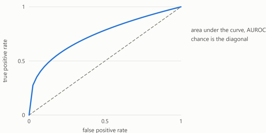
Figure 188: Twice the held-out AUROC minus one, or zero.
