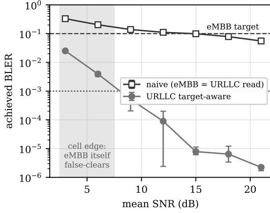
Fig. 2. The target gap across mean SNR (real NR, Sionna LDPC; sealed sweep, 3 seeds, whiskers min-max). The naive certificate rides the eMBB target, so the URLLC consumer sees roughly a hundredfold false-clear at every in-range SNR. Below about 6 dB (shaded) even the eMBB consumer is failed. The target-aware policy holds URLLC throughout.
