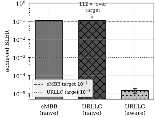
Fig. 1. One report, two verdicts (real NR, Sionna LDPC; 3 sealed seeds, 6000 TTI each; bars are means, whiskers min-max). The same CSI-derived MCS meets the eMBB target and misses the URLLC target by 112 \times . The target-aware policy meets URLLC.
