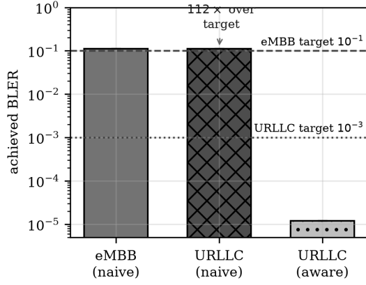
Fig. 1. Consumer-relativity of the CSI certificate in the reliability target (real NR, Sionna LDPC; three sealed seeds). The identical CSI-derived MCS meets the eMBB target ( 10^{-1} ) but false-clears the URLLC target ( 10^{-3} ) by 112\times ; a target-aware policy meets URLLC at the cost of \sim 2 dB margin.
