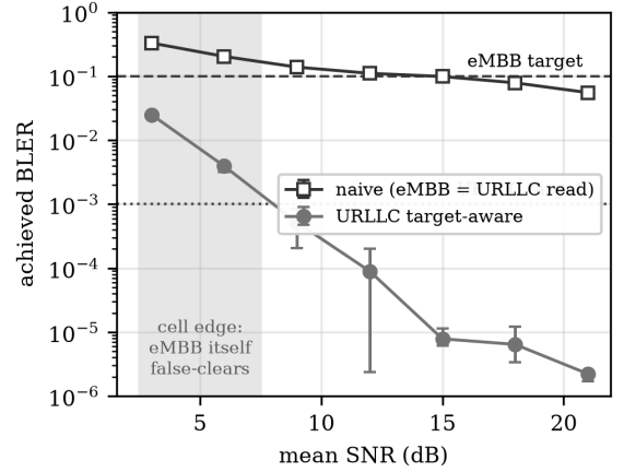
Fig. 1. The target gap across mean SNR (real NR, Sionna LDPC; sealed sweep, 3 seeds, whiskers min-max). The naive certificate rides the eMBB target, so the URLLC consumer sees roughly a hundredfold false-clear at every in-range SNR. Below about 6 dB (shaded) even the eMBB consumer is failed. The target-aware policy holds URLLC throughout.
