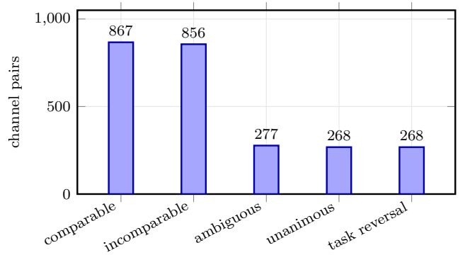
FIG. 2. The declared ensemble of 2000 random leakage channel pairs. The first three bars partition the ensemble by certificate, comparable when a garbling is certified in some direction, incomparable when both searches are refused above the declared 0.01, ambiguous otherwise and excluded as declared. The last two bars are subsets of the incomparable class, pairs ordered unanimously by all seven declared divergences and pairs whose unanimous ordering is reversed by a task in the declared battery. The two subsets are equal at 268. No comparable pair carries a reversal. Every count is read from the committed evidence record.
