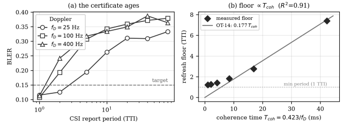
Fig. 3. The CSI certificate's refresh horizon (real NR, Sionna LDPC; sealed sweep). (a) The certificate ages: BLER grows with report period, faster at higher Doppler. (b) The refresh floor is proportional to the Clarke coherence time ( 0.177 T_{\text{coh}} , R^2 = 0.915 ); at high Doppler it saturates at one TTI.
