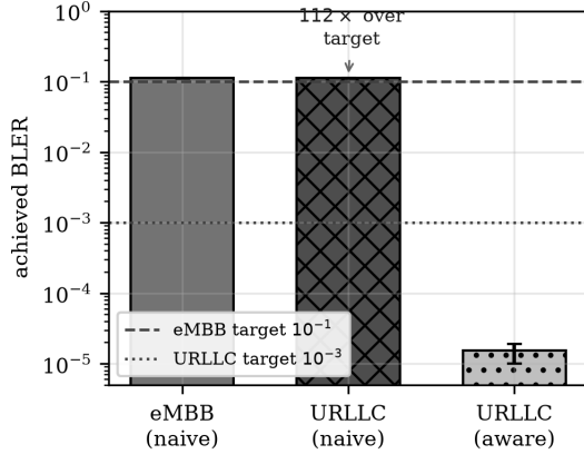
Fig. 2. Consumer-relativity of the CSI certificate in the reliability target (real NR, Sionna LDPC; 3 sealed seeds, T=6000 TTI each; bars are means, whiskers min-max). The identical CSI-derived MCS meets the eMBB target ( 10^{-1} ) but false-clears the URLLC target ( 10^{-3} ) by 112\times ; a target-aware policy (conservative MCS + K=3 independent diversity branches) meets URLLC.
