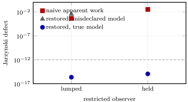
FIG. 3. The defect ladder and its restoration. The lumped observer's naive Jarzynski defect is 4.33 \times 10^{-4} and the held observer's is 0.0324, while the complete and blind observers' defects are exactly zero and sit off this logarithmic scale. Bayes work estimates filtered through the true declared detector model restore both identities below the dashed declared bar of 10^{-12} , to 2.2 \times 10^{-16} and 1.1 \times 10^{-15} . The same filter built from a misdeclared model, kernels at inverse temperature 0.9, leaves the lumped observer at 3.27 \times 10^{-3} , a larger defect than no correction at all. Every point is read from the committed evidence records.
