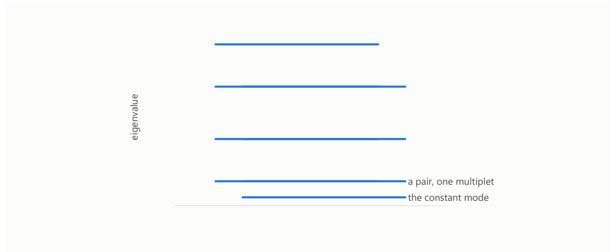
Figure 139: Eigenvalues that come in equal groups.
