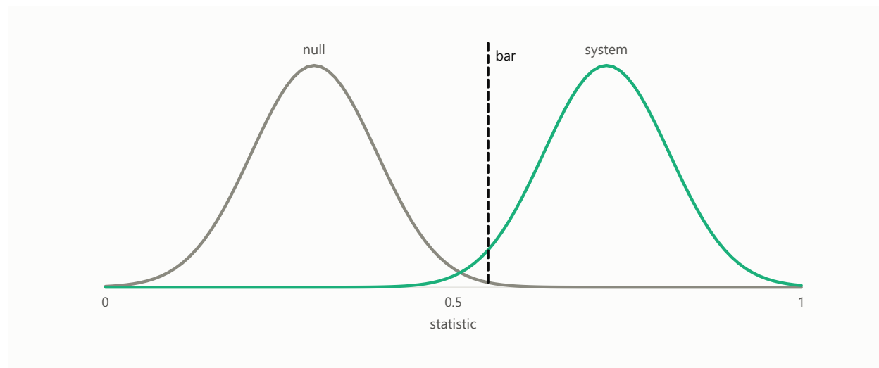
Figure 19: A bar discriminates when the null fails it and the system passes it.
