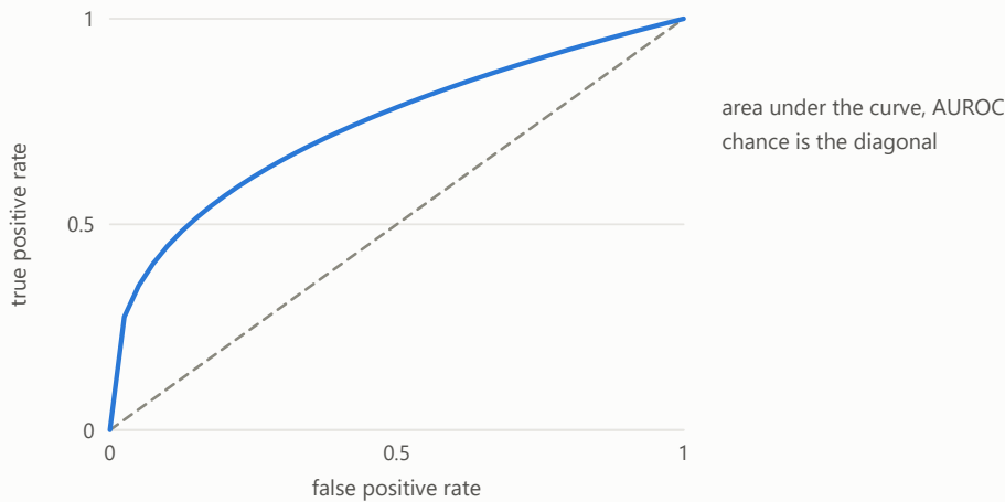
Figure 15: The area under the curve is the chance that a random positive outscore a random negative.
