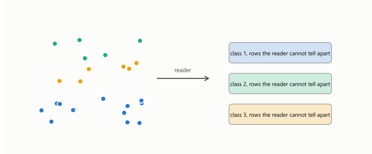
Figure 17: Documents with the same counts are the same document to the reader, whatever the order.
