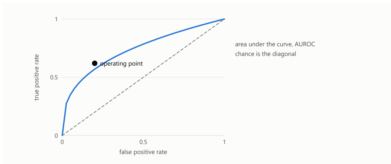
Figure 148: The row at which a consumer is read, or the threshold at which a classifier is scored.
