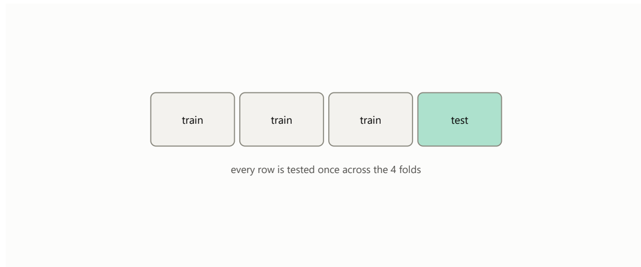
Figure 213: The rows a model is fit on and the rows it is scored on.
