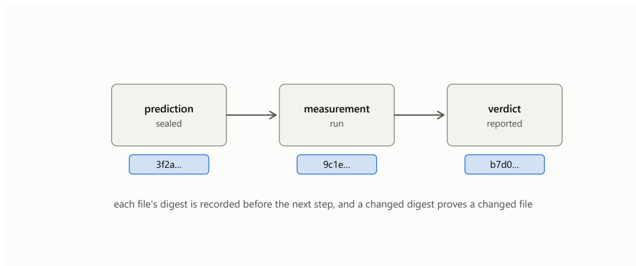
Figure 186: Written into a sealed file before the measurement.
