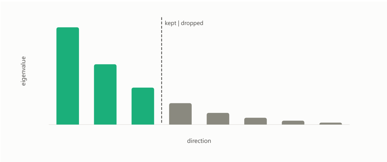
Figure 229: The first k components kept and the rest dropped.
