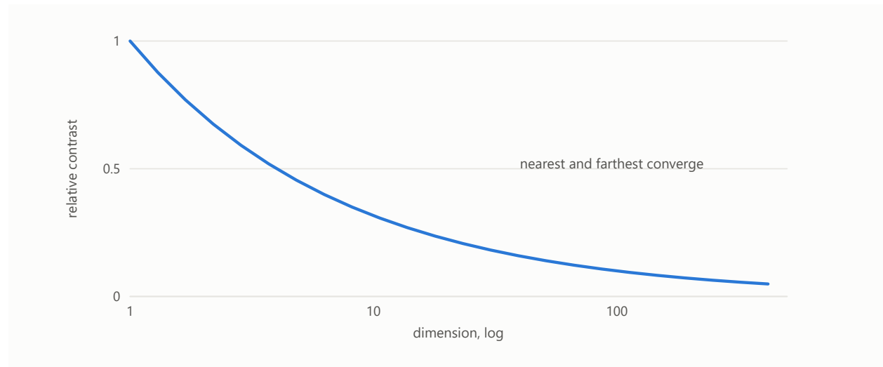
Figure 71: Nearest and farthest converge as the dimension grows.
