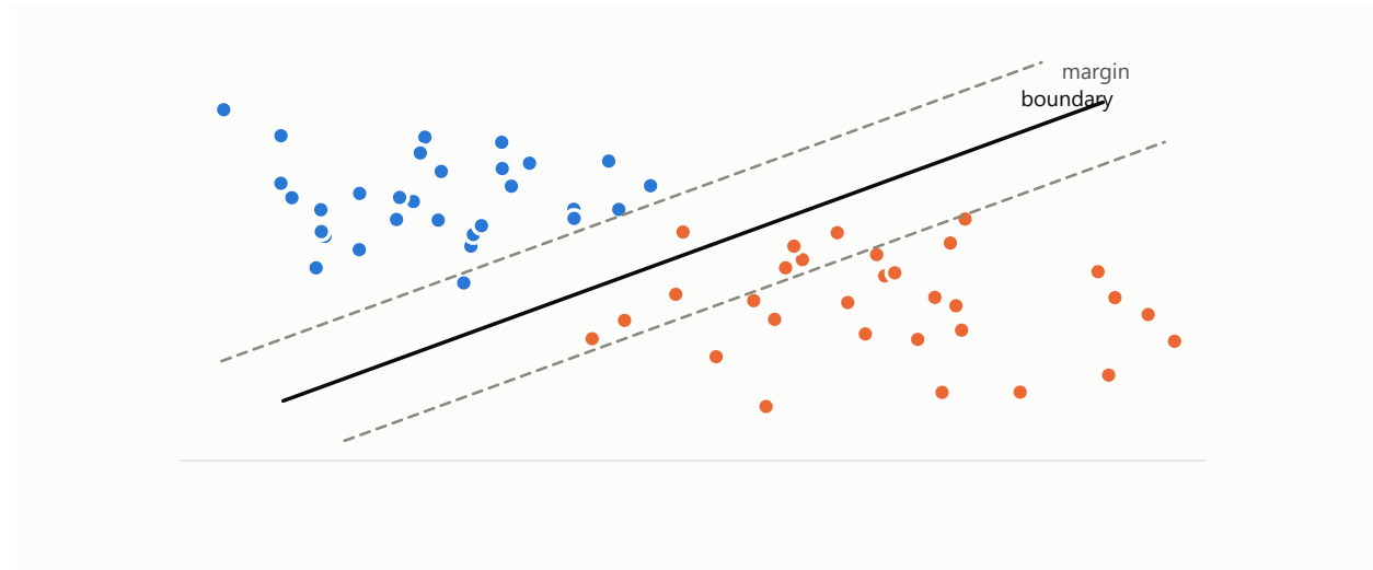
Figure 129: A weighted sum, whose boundary is a hyperplane.
