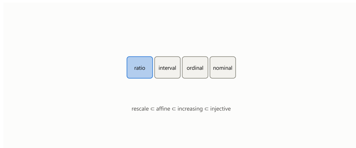
Figure 12: The four scales and the transformations each permits, nested from ratio to nominal.
