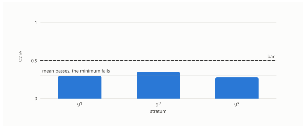
Figure 205: Every group shows one sign and the aggregate shows the other.
