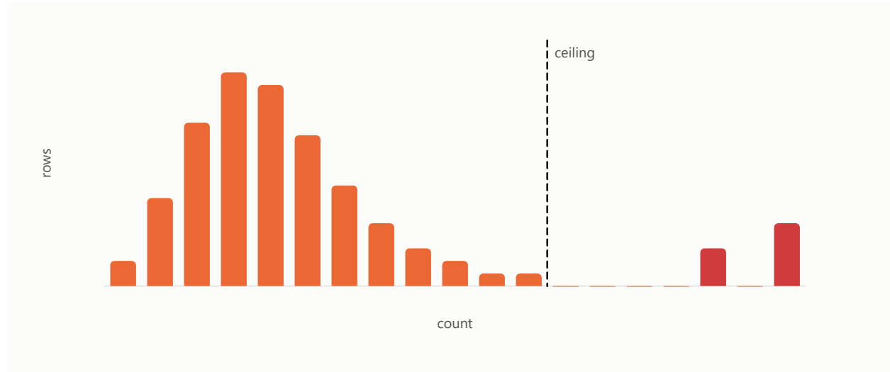
Figure 106: The count distribution's tail above the Poisson ceiling.
