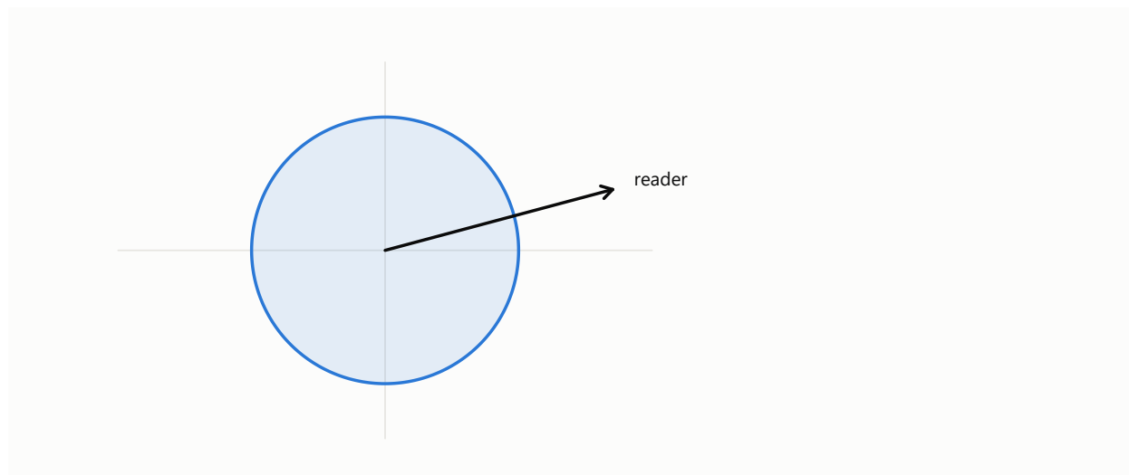
Figure 112: Every direction has the same variance.
