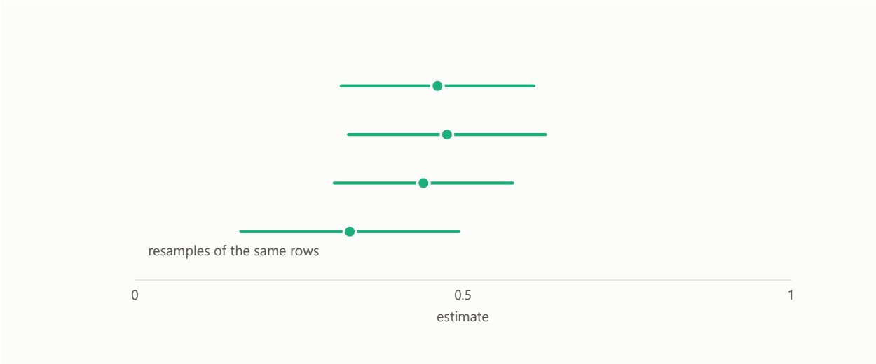
Figure 16: Resamples of the same rows, each fit and then averaged.
