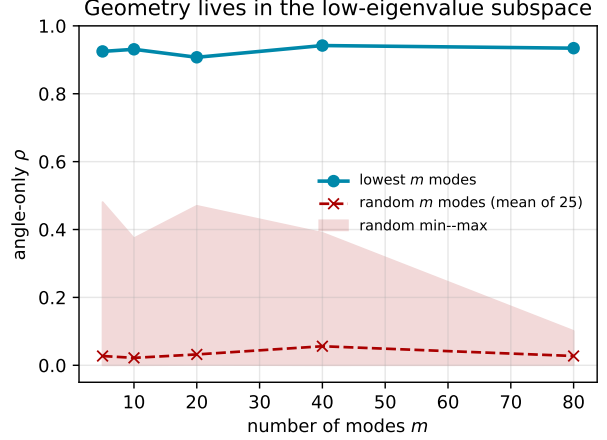
Figure 2: Geometry lives in the low-eigenvalue subspace: lowest- m modes preserve geodesics; a random-mode basis of equal size does not. The random curve is the mean over 25 draws, the band its full min-max envelope—even the best-case random draw stays far below the low-mode curve.
