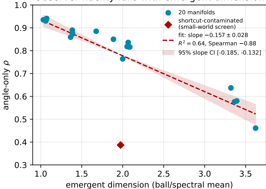
Observer fidelity falls with emergent dimension
