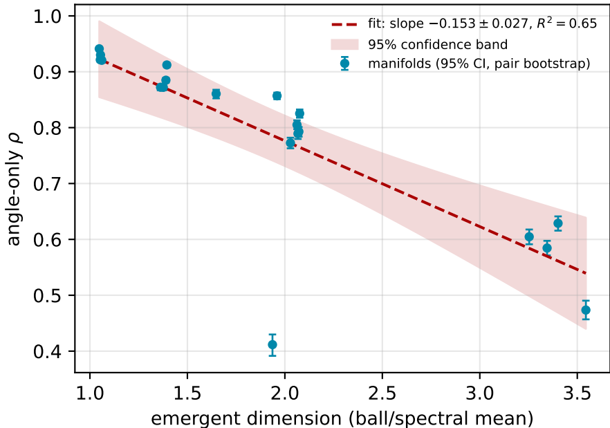
Angular fidelity vs emergent dimension (20 manifolds)
