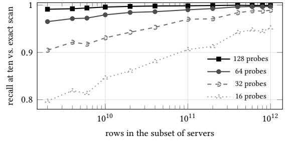
Figure 2: Recall against the exact scan of k servers of the one index, mean of five random subsets, from two billion to a trillion rows. Wide probes are flat, and narrow probes gain as rows are added.
