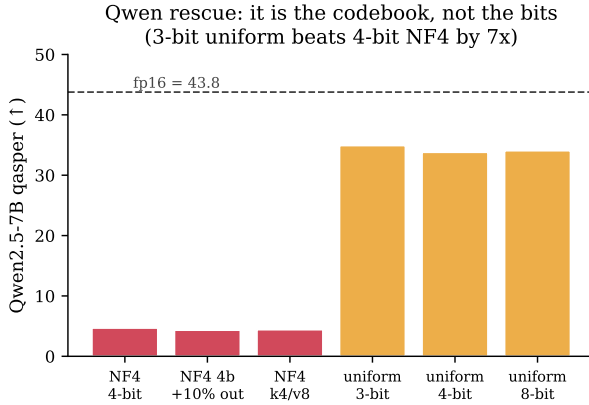
Figure 3: Qwen rescue sweep. The codebook—not the bit budget—decides survival.
