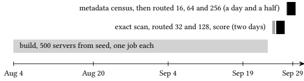
Figure 2: The run on the calendar. The index was built over seven weeks by a pool of one job per server. The measurement, the census and the second sweep took four days at the end of September, all through the same controller.
