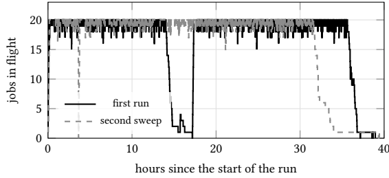
Figure 3: Jobs the pool had in flight, from the driver logs, for the first run (exact scan, routed passes at 32 and 128 probes, score) and the second sweep (routed passes at 16, 64 and 256 probes, score). The pool holds the controller’s cap of twenty until each phase drains.
