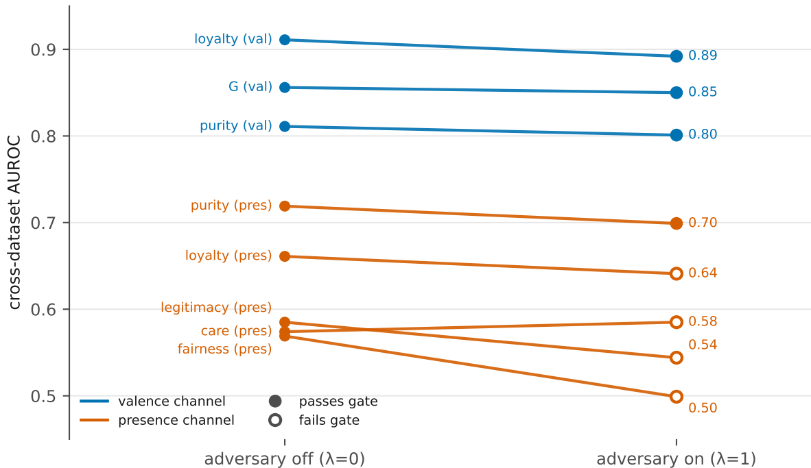
Valence transfers regardless of the adversary; identity does not
