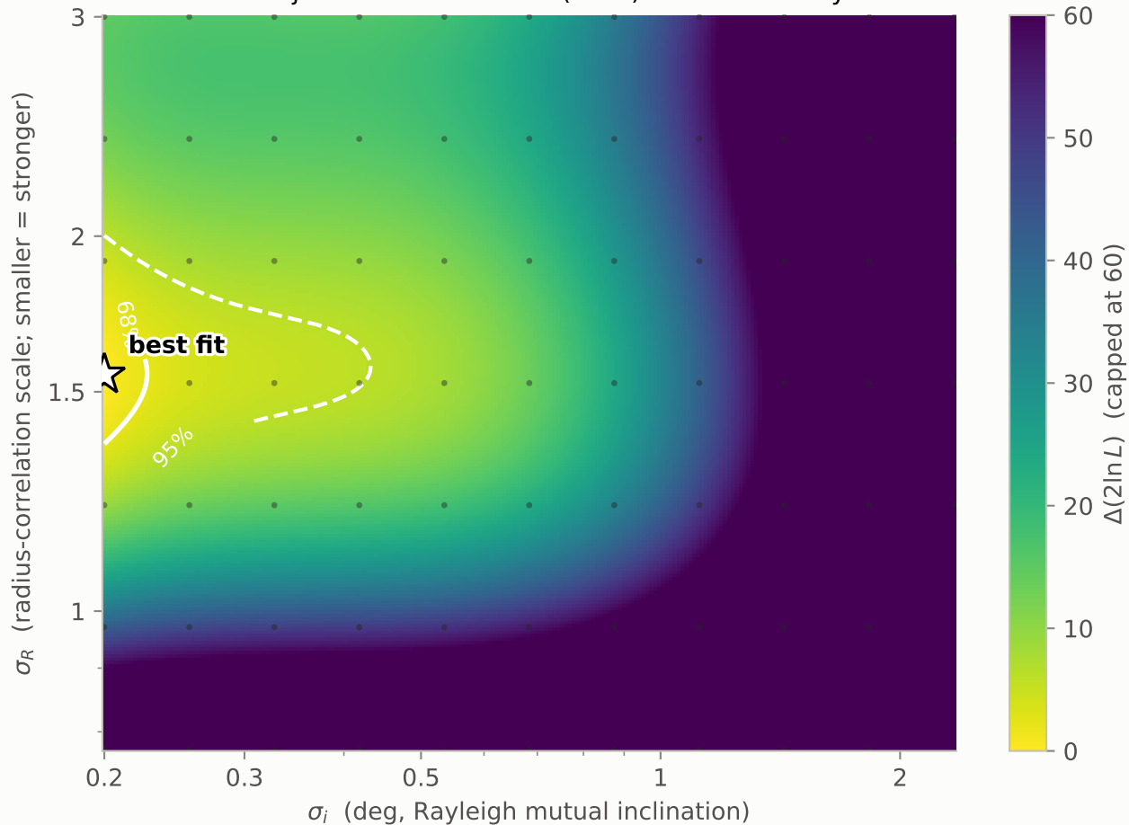
DR25 joint fit: smoothed \Delta(2\ln L) over the valley
