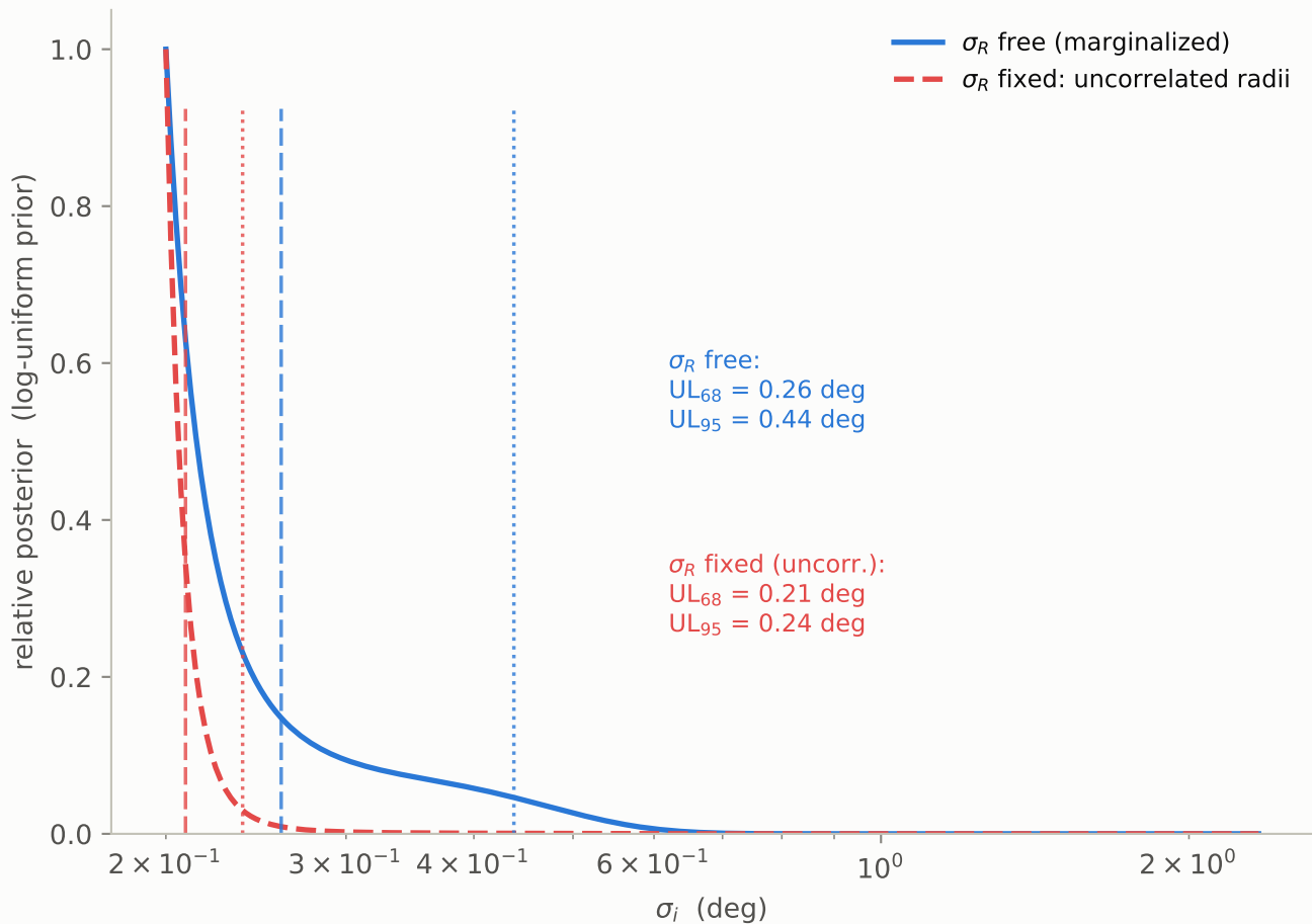
\sigma_i marginal posterior: joint vs radius-independent model
