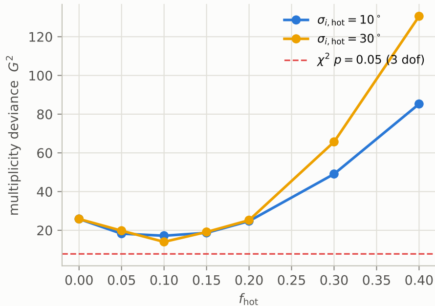
Multiplicity goodness of fit
