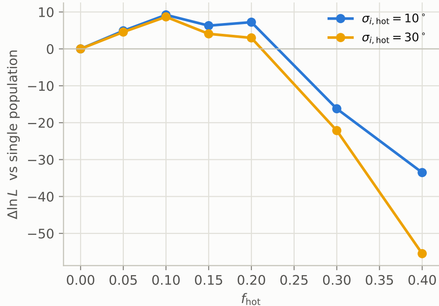
Mixture likelihood gain
