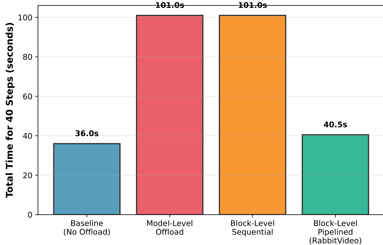
(a) Total Inference Time Comparison
