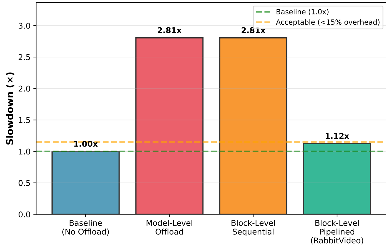
(b) Slowdown Comparison
