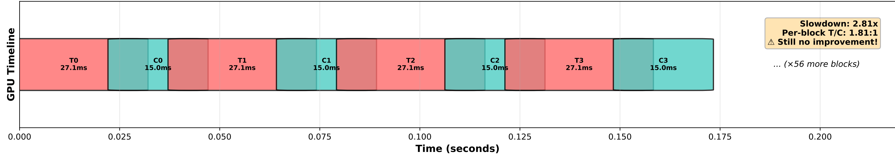
(c) Block-Level Pipelined (RabbitVideo): Overlap Transfer[i+1] with Compute[i]
