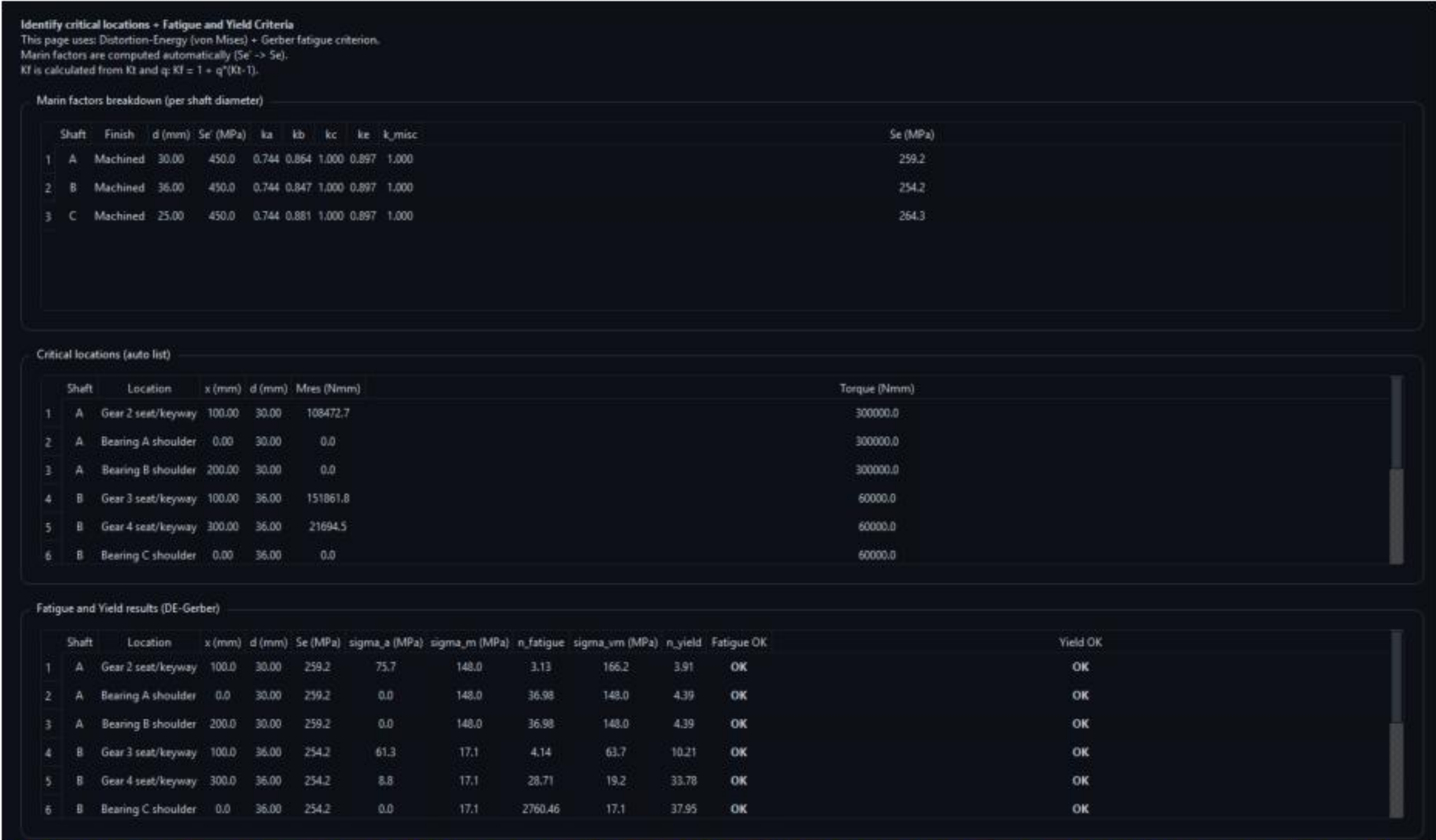
Figure 7: Automated Fatigue and Yield safety factor calculations showing compliance with DE-Gerber criteria.
