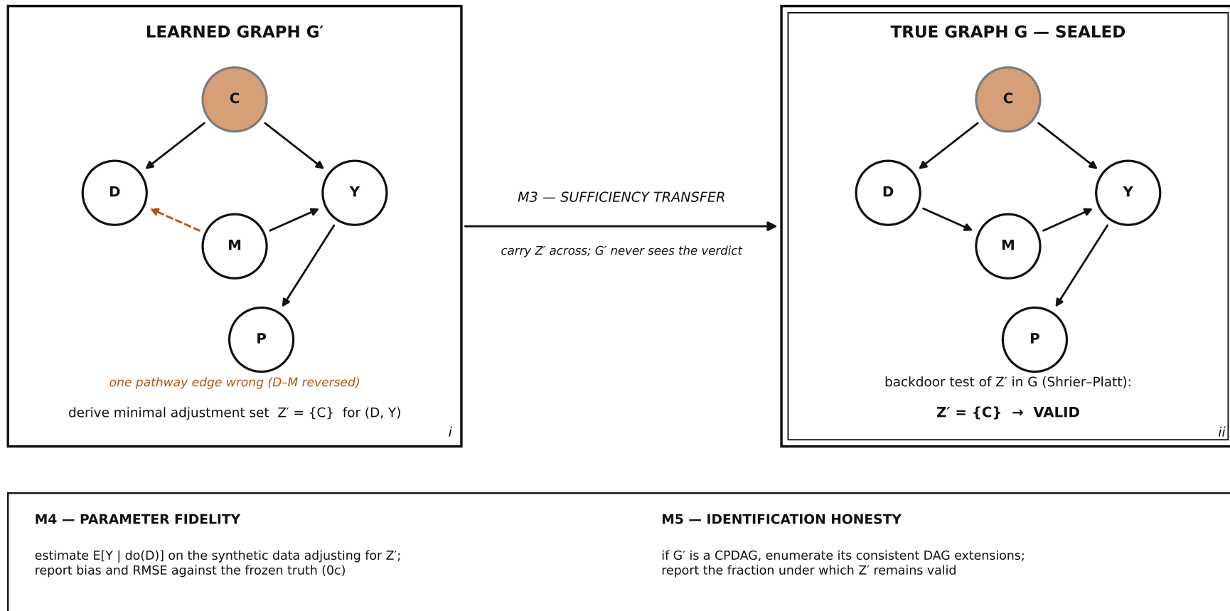
FIG. 2 — topological error and functional failure are different events: G' is wrong about the pathway yet sufficient for the target parameter
