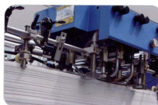
Paper feeding system
