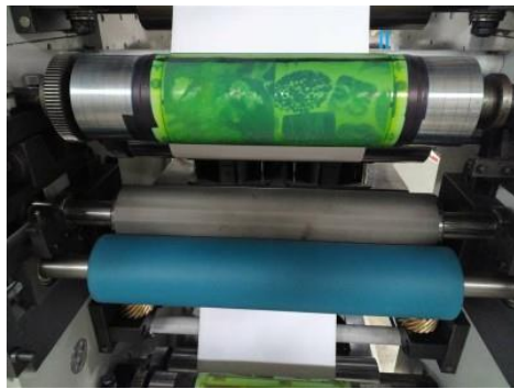
Ink roller, anilox, plate roller
