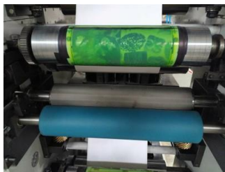
Ink roller, anilox, plate roller
