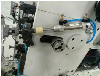
Separation of plate roller and anvil roller
