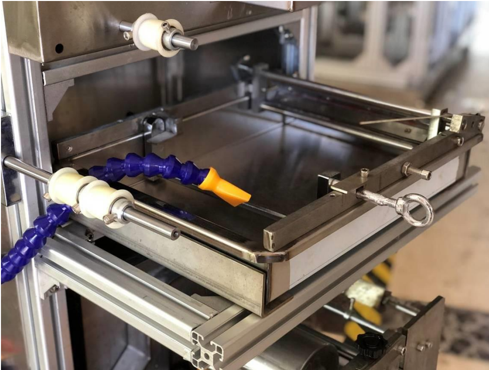
Top Layer – Single side glue
