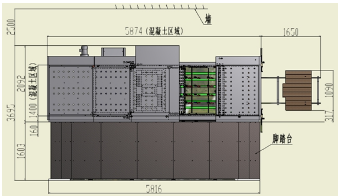
Foundation Diagram 2
