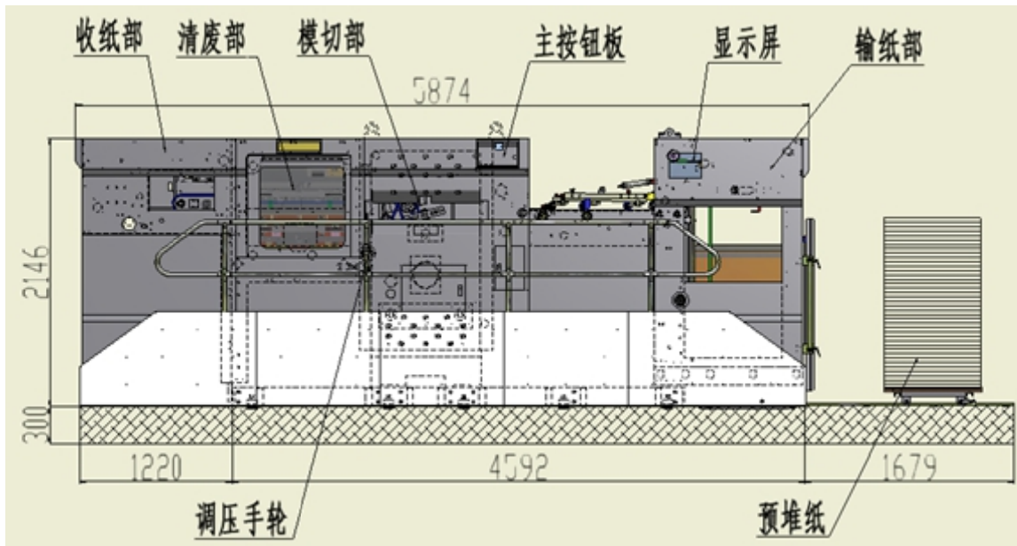
Ground Schematic 1
