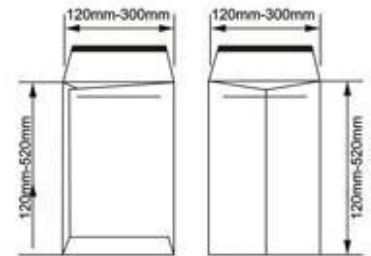
纸袋加工尺寸规格 Paper size envelope film sticked process
