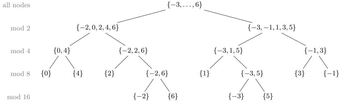
Figure 11.1: The tree of residue classes of the nodes \mathcal{N} = \{-3, \dots, 6\} ( n = 3 ) for p = 2 . A node becomes a leaf at the first level where its class has one element. For two nodes k \neq m , v_2(k - m) is the level of their lowest common class: -2 and 6 separate at level 4 and v_2(8) = 3 ; 0 and 4 separate at level 3 and v_2(4) = 2 ; 0 and 1 separate at level 1 and v_2(1) = 0 .
