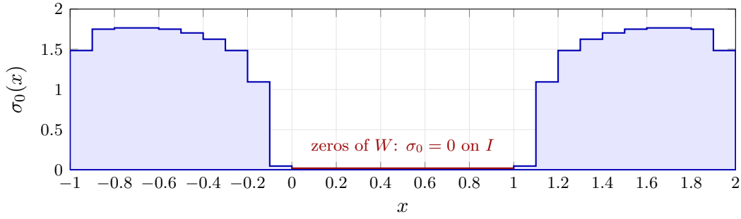
Figure 10.2: The trial density \sigma_0 [note, (5.9)], symmetric about x = \frac{1}{2} . Its mass is m_0 = \frac{463}{160} and its maximum \frac{113}{64} \approx 1.77 , far below the cap 4.
