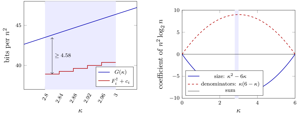
Figure 7.1: Left: the gain coefficient G(\kappa) (bits per n^2 ) on the range [2.8, 3] (shaded), against the note's upper bounds for F_i^\dagger + c_i on the five intervals (sums of the entries of [note, Table 1]: 38.91, 39.25, 39.62, 39.99, 40.37). The gap between the curve and the steps is the margin; it is smallest at the left end of I_1 , where it is 43.49 - 38.91 = 4.58 . Right: the two main terms of order n^2 \log_2 n . They are exact negatives of each other for every \kappa , so their sum is identically 0. Each is about 9 n^2 \log_2 n bits on the shaded range, about 90 n^2 bits for n = 1000 (Chapter 1), many times the final margin of 4.58 n^2 .
