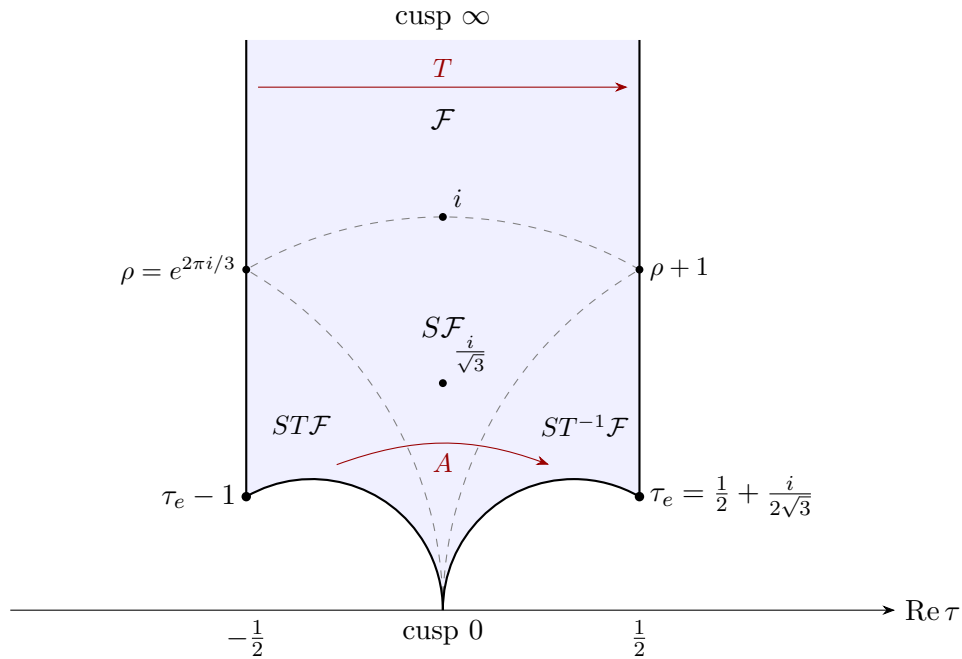
Figure 16.1: The fundamental domain \mathcal{F}_3 of \Gamma_0(3) (shaded, bold boundary), the union of four copies of the standard domain \mathcal{F} of \mathrm{SL}_2(\mathbb{Z}) (dashed lines separate the copies). T glues the two vertical sides, A = \begin{pmatrix} 1 & 0 \\ 3 & 1 \end{pmatrix} glues the left arc |\tau + \frac{1}{3}| = \frac{1}{3} to the right arc |\tau - \frac{1}{3}| = \frac{1}{3} . The domain touches the real axis only at the cusp 0; the two lower corners \tau_e - 1 and \tau_e are glued by T and form one elliptic point.
