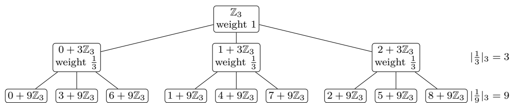
Figure 4.1: \mathbb{Z}_3 as a tree of balls. Level N consists of the 3^N balls t + 3^N\mathbb{Z}_3 , 0 \leq t < 3^N , each represented by its smallest non-negative integer t . The Riemann sum S_N gives each ball the weight 3^{-N} and evaluates f at its representative. The weights add up to 1 at every level, but each individual weight is 3-adically large, |3^{-N}|_3 = 3^N .
