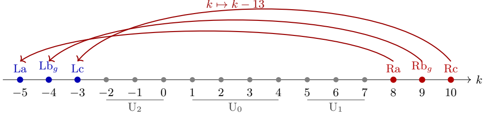
Figure 14.1: n = 5, p = 13 : the nodes -5, \dots, 10 with their types (Example 14.7); arrows join each R node to its partner.
