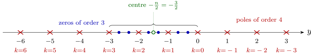
Figure 5.1: The weight W for n = 3 on the real line. Crosses: the poles of order 4 at the integers y = -k , labelled by their node k \in \{-3, \dots, 6\} (note the sign). Filled dots: the zeros -(j + \frac{r}{3}) of order 3, j = 0, 1, 2 , r = 1, 2 , all in the interval (-3, 0) . Open circle: the simple zero at y = -\frac{3}{2} , the centre of the ten poles, which is not a node because n is odd. The antisymmetry W(-n - y) = -W(y) is the reflection of this picture about -\frac{3}{2} .
