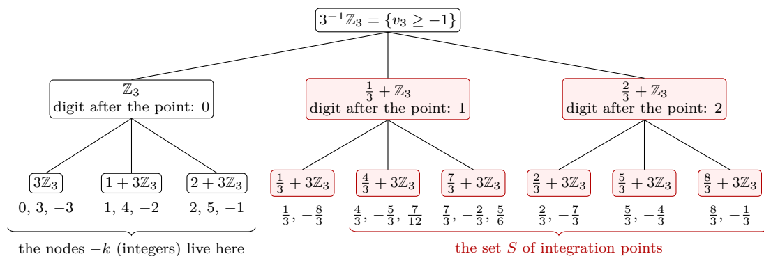
Figure 2.1: The set 3^{-1}\mathbb{Z}_3 as a tree of digits. Each node of the tree is a ball (a set c + 3^j\mathbb{Z}_3 ); going down one level fixes one more digit, starting from the rightmost one, a_{-1} (after the point), and moving left to a_0 , a_1 , and so on (only the first two levels are drawn, with sample elements). Two numbers are at distance 3^{-j} when a_j is the rightmost digit at which they differ: numbers in different boxes of the first level are at distance 3, numbers in different boxes of the second level below the same first-level box are at distance 1. The set S (red) is the two right branches at the top level; all integers, in particular all nodes -k of the weight, are in the left branch. Hence every point of S is at distance exactly 3 from every node ( Proposition 2.31 ).
