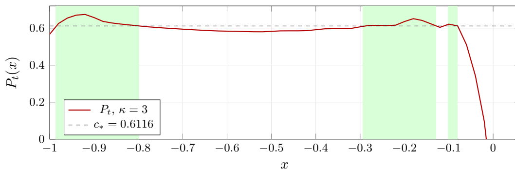
Figure 10.3: P_t on [-1, 0.06] for \kappa = 3 (the picture on [0.94, 2] is the mirror image). Shaded: the set \{P_t > c_*\} on which the bathtub puts density 4, of total length \frac{3}{4} on both sides together (fine grid, floating point, no modulus term). The kinks at multiples of 0.1 come from the jumps of \sigma_0 . Sampled every 0.02.
