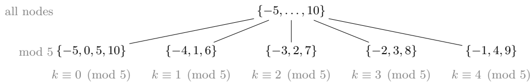
Figure 11.2: The same for n = 5 ( \mathcal{N} = \{-5, \dots, 10\} ) and p = 5 . Since 25 > 3n = 15 , every class modulo 25 is a single node: the tree has one level below the root, and v_5(k - m) \in \{0, 1\} for all pairs of nodes.
