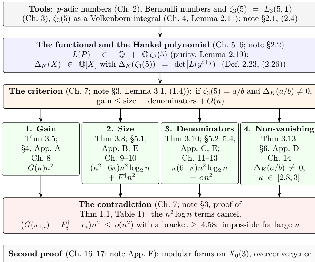
Figure 1.1: The structure of the proof of [note, Theorem 1.1]. Chapter numbers refer to this companion, section, lemma and theorem numbers to the note. The criterion supplies the inequality, the four estimates fill in its terms, and Table 1 closes the argument. The second proof shares only the statement and the normalization [note, (2.4)] with the first.
