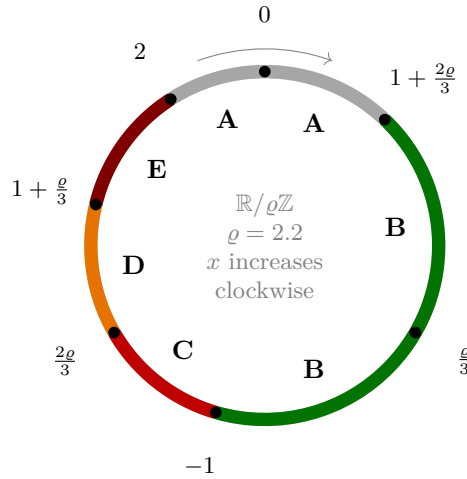
Figure 13.1: The circle \mathbb{R}/\rho\mathbb{Z} for \rho = 2.2 , with the seven points (13.8) (angle 90^\circ - 360^\circ x/\rho ) and the type of each arc (Example 13.9). Grey (A): one node with a p -special zero only. Green (B): one node, no cost. Red and orange (C, D, E): two nodes with partners, where the losses sit. Every class of every prime p with p/n \in (2, \frac{9}{4}) is a point of this picture.
