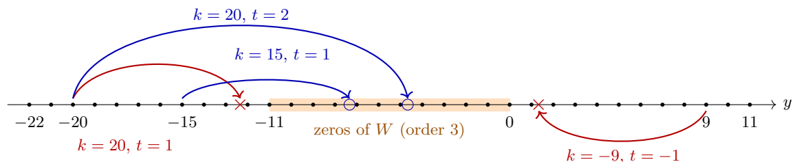
Figure 12.1: n = 11 , p = 23 , in the variable y of W : the nodes y = -k (dots, k = -11, \dots, 22 ) and the comb of triple zeros on \frac{1}{3}\mathbb{Z} \setminus \mathbb{Z} inside (-11, 0) (shaded). An arrow goes from a node to one of its virtual poles y = -k + \frac{23t}{3} . Circles: covered (the point is a triple zero of W ); crosses: uncovered. The node k = 15 has one virtual pole, covered; k = 20 has two, t = 2 covered and t = 1 at y = -\frac{37}{3} outside the comb; k = -9 has one at y = \frac{4}{3} > 0 , uncovered.
