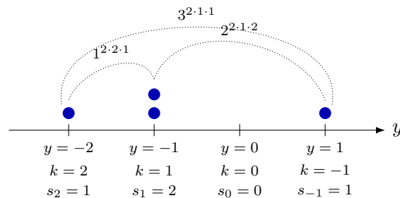
Figure 9.1: The profile s = (1, 0, 2, 1) for n = 1 , K = 4 : the four “particles” y_1, \dots, y_4 placed at the nodes. The leading part of the cross factor is \prod_{k < m} |k - m|^{2s_k s_m} = 2^4 \cdot 1^4 \cdot 3^2 = 144 ; each node with s_k \geq 1 contributes a local factor built from its own local constants.
