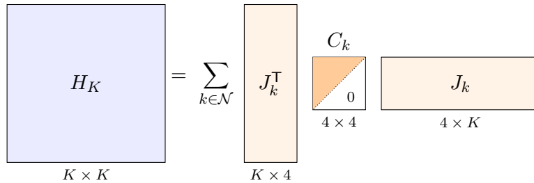
Figure 6.1: The jet form (6.3): the K \times K Hankel matrix is a sum of 3n+1 terms, one per node, each passing through the 4 \times 4 matrix C_k of local constants, which is zero below its anti-diagonal (shaded: the entries c_{k,a+b} with a+b \leq 3 ). Each term has rank at most 4.
