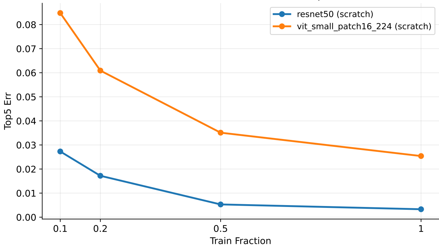
[Scratch] ResNet vs ViT — TEST Top5 Err
