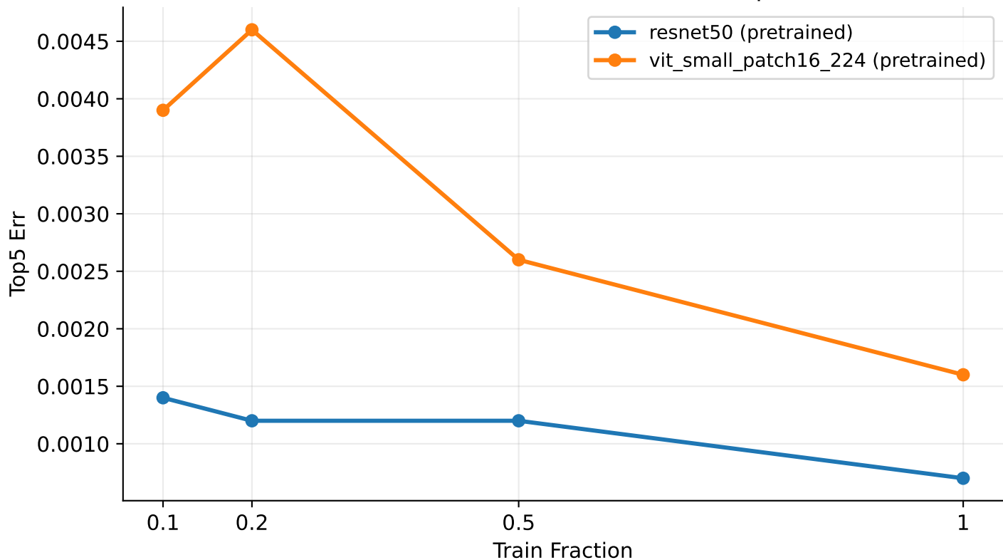
[Pretrained] ResNet vs ViT — TEST Top5 Err
