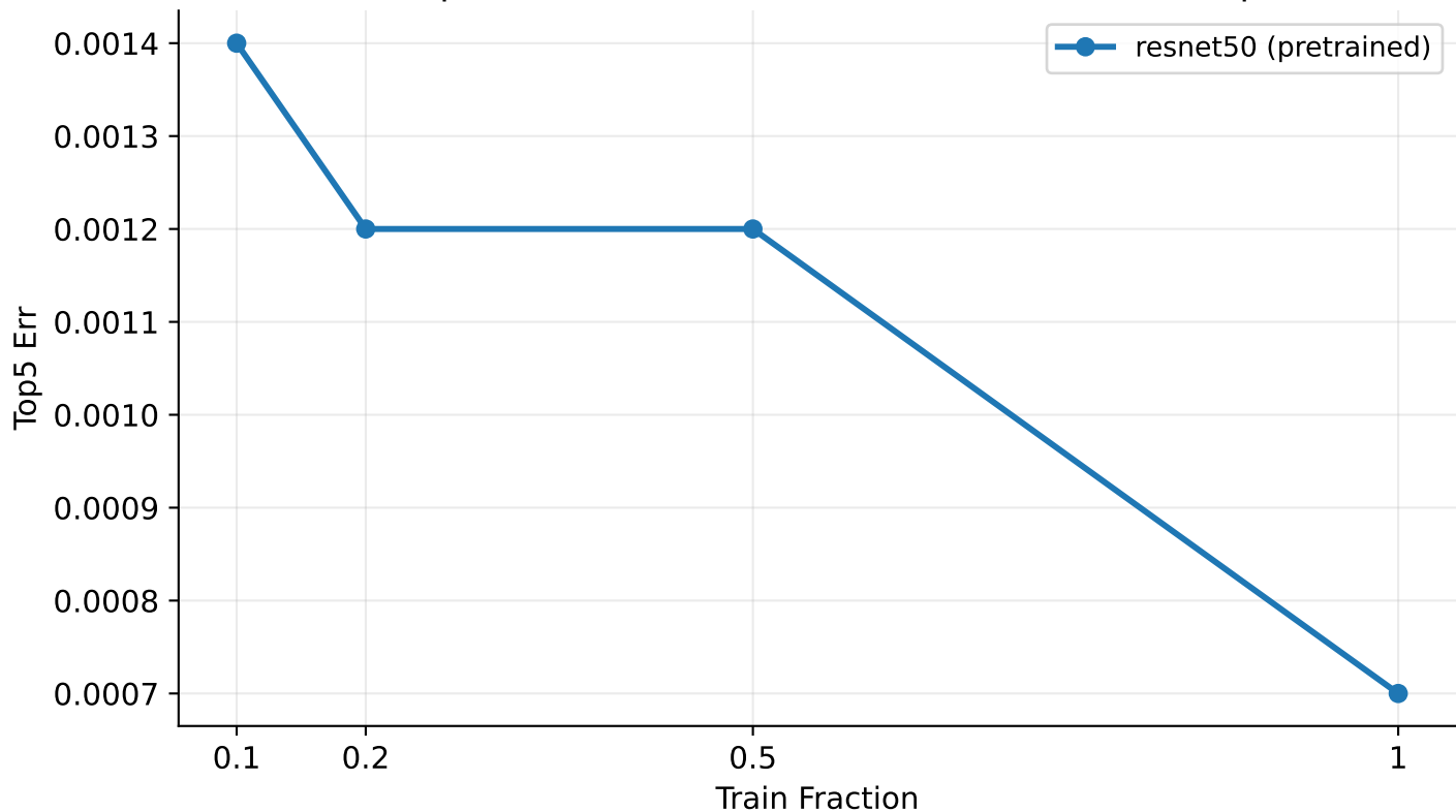
[ResNet pretrained] Error vs Train Fraction — TEST Top5 Err
