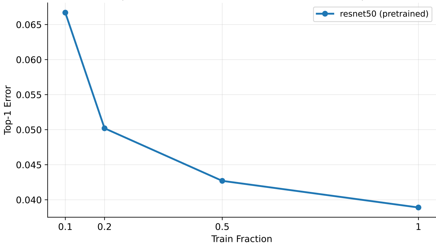
[ResNet pretrained] Error vs Train Fraction — TEST Top-1 Error
