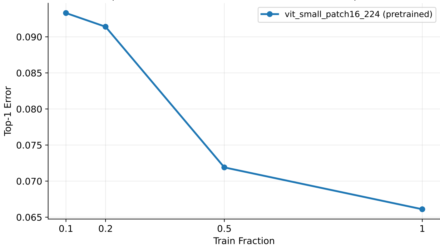
[ViT pretrained] Error vs Train Fraction — TEST Top-1 Error
