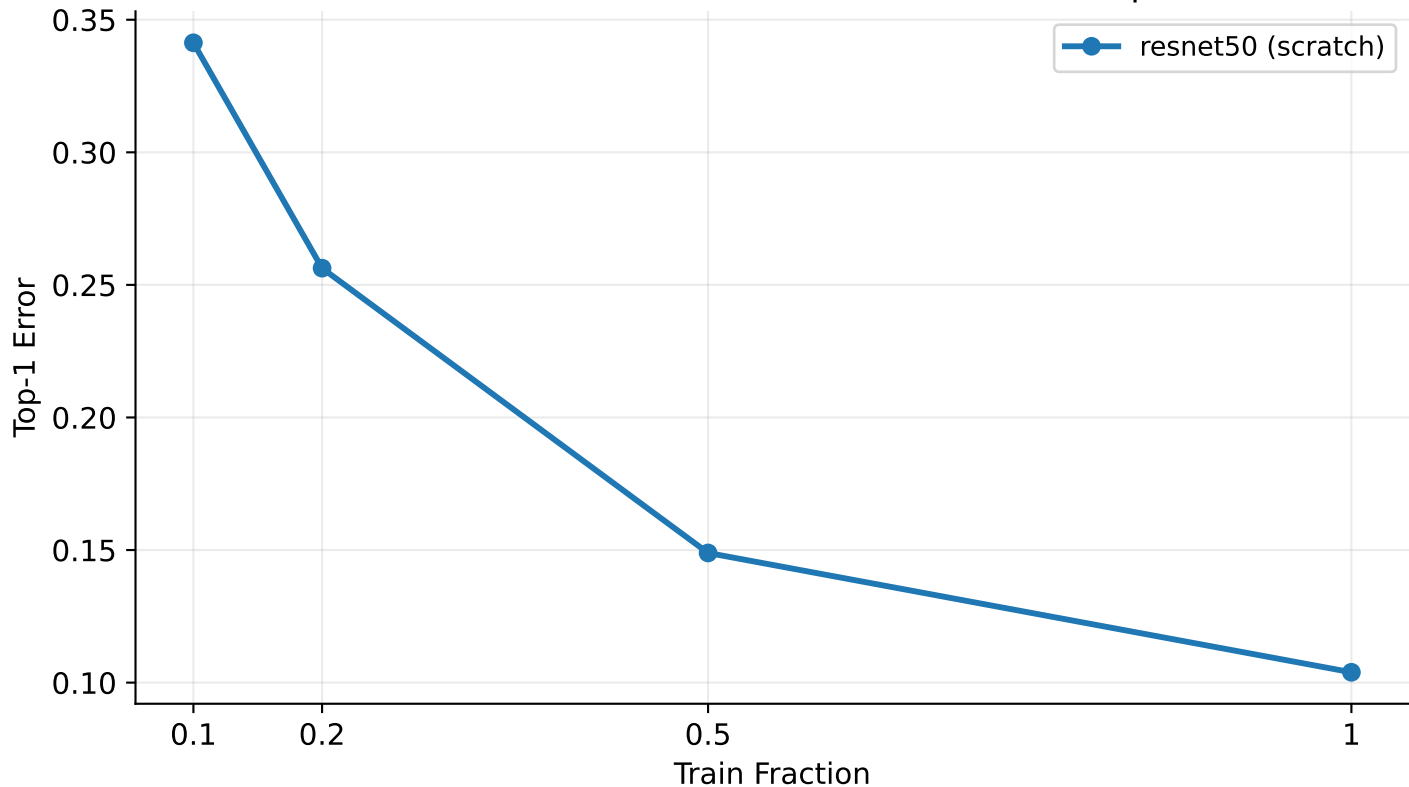
[ResNet scratch] Error vs Train Fraction — TEST Top-1 Error
