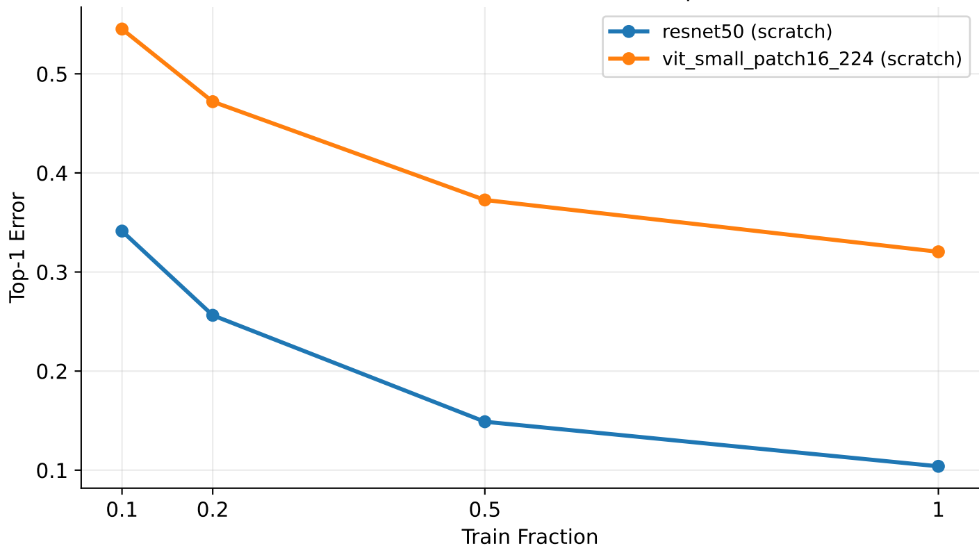
[Scratch] ResNet vs ViT — TEST Top-1 Error
