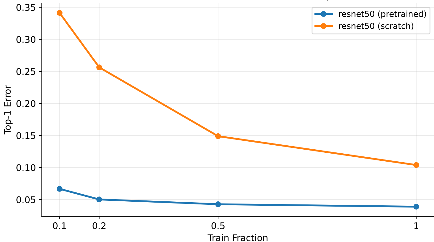
[ResNet] Pretrained vs Scratch — TEST Top-1 Error
