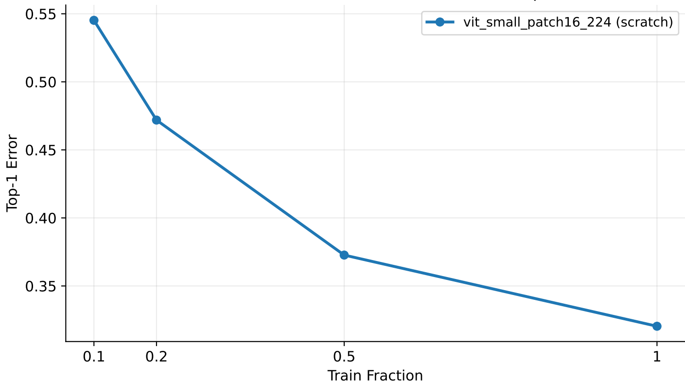
[ViT scratch] Error vs Train Fraction — TEST Top-1 Error
