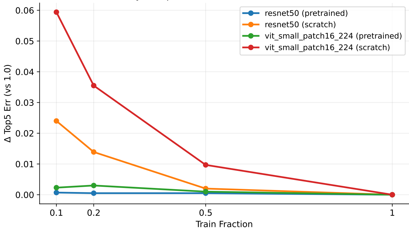
[Sensitivity] \Delta Top5 Err vs Train Fraction (relative to 1.0)
