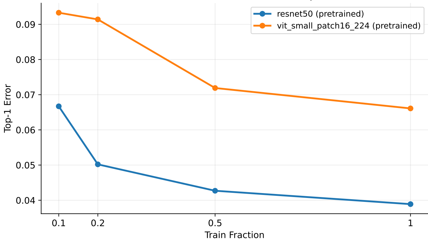
[Pretrained] ResNet vs ViT — TEST Top-1 Error
