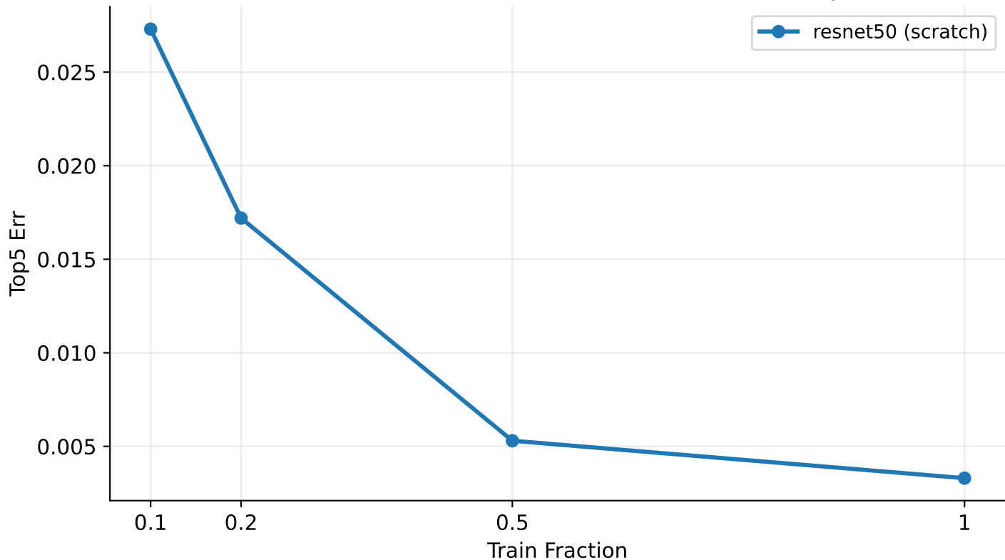
[ResNet scratch] Error vs Train Fraction — TEST Top5 Err
