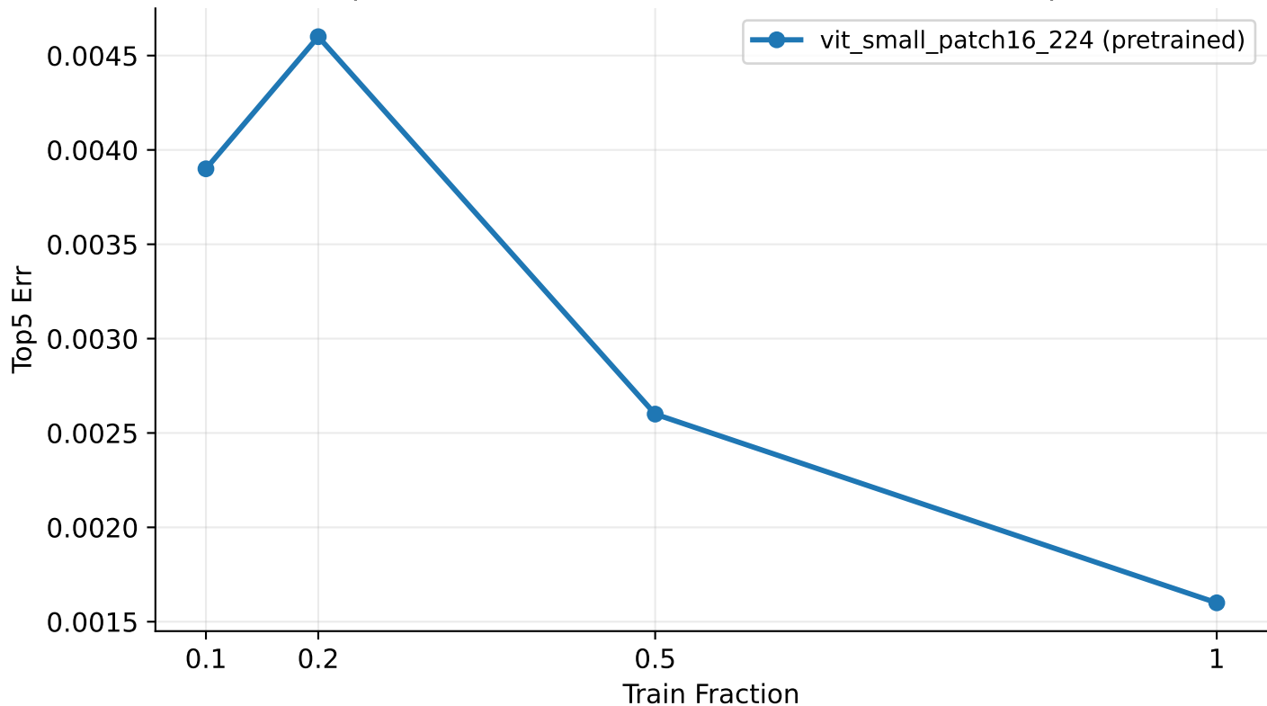
[ViT pretrained] Error vs Train Fraction — TEST Top5 Err
