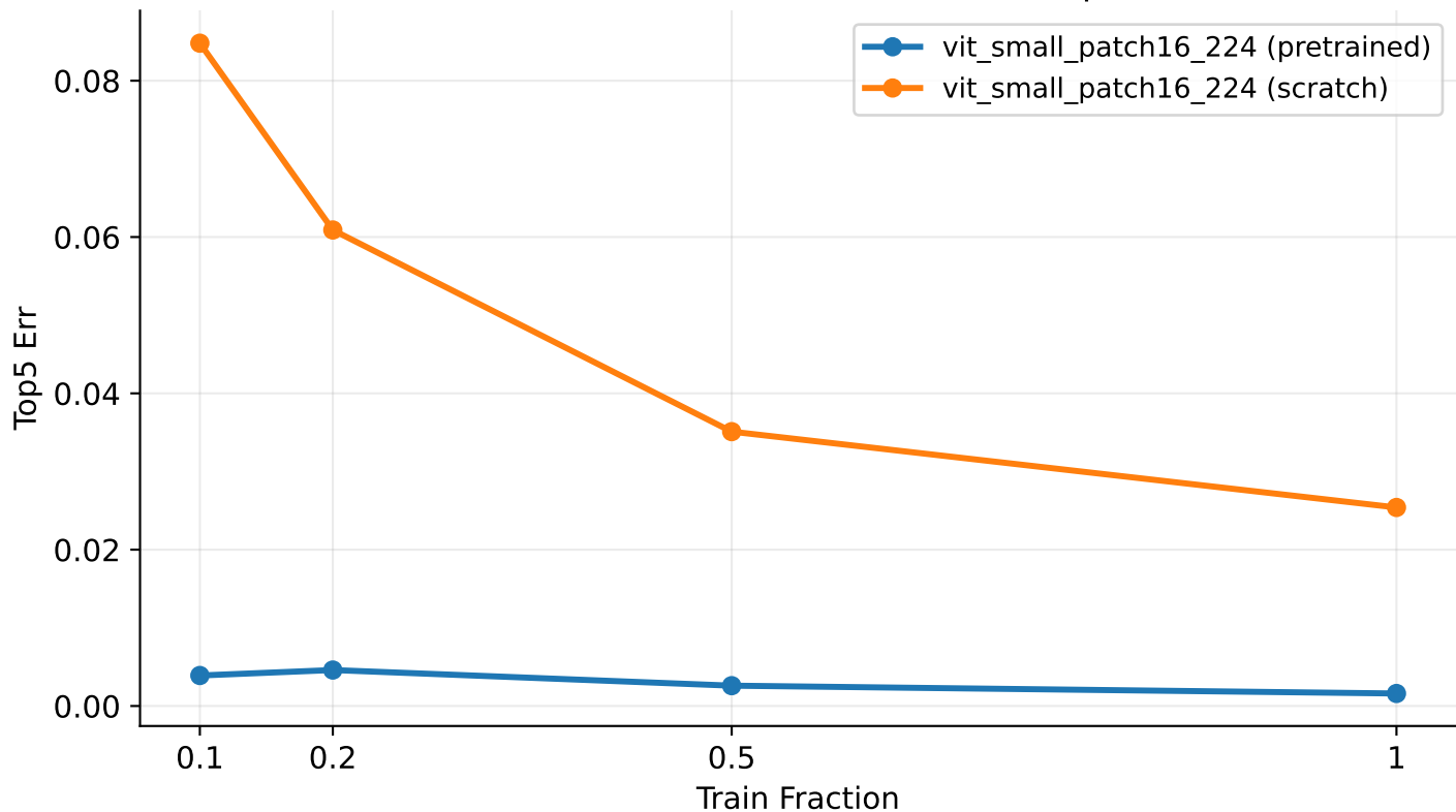
[ViT] Pretrained vs Scratch — TEST Top5 Err
