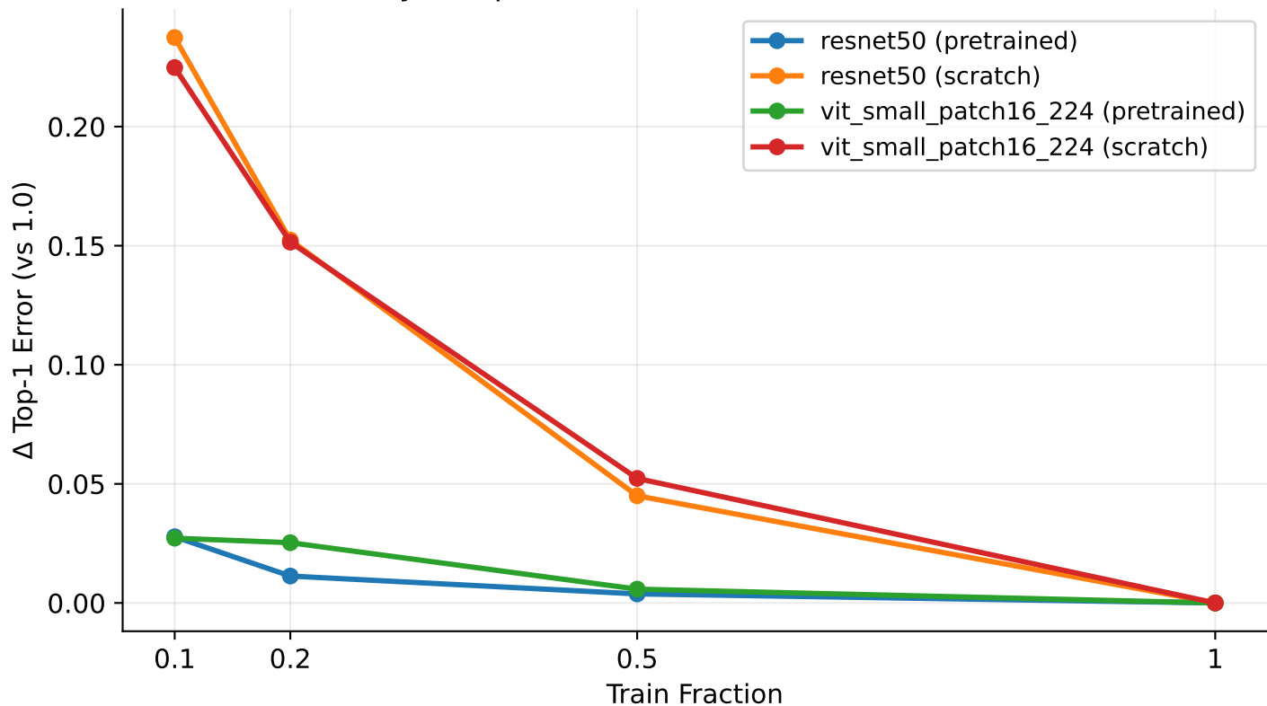
[Sensitivity] \Delta Top-1 Error vs Train Fraction (relative to 1.0)
