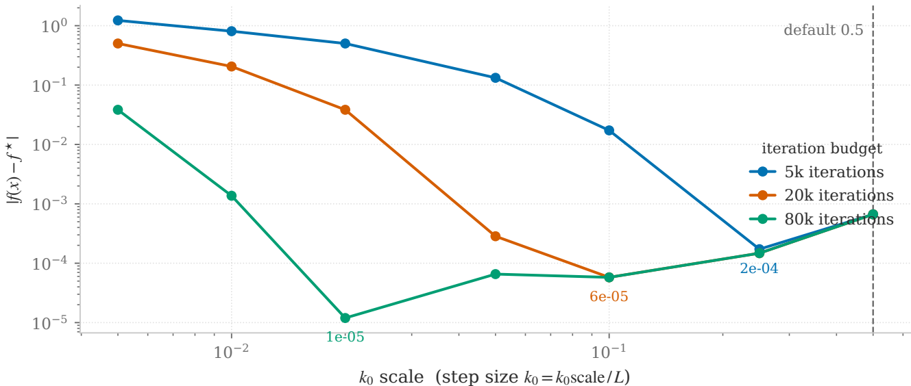
Accuracy of the fixed point vs step size, at three iteration budgets 50-D QP with 30 inequalities (the Figure 1 problem)
