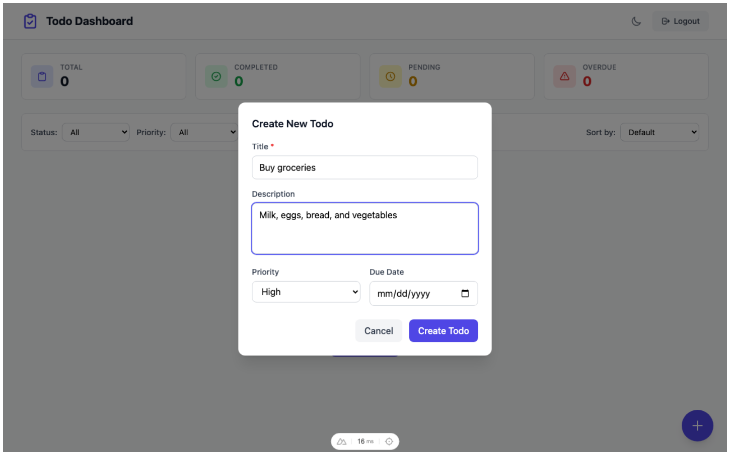
Figure: Dashboard Modal Create Todo Filled
