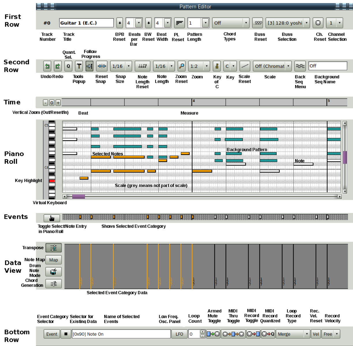
Figure 32: Pattern Editor Window, Annotated
