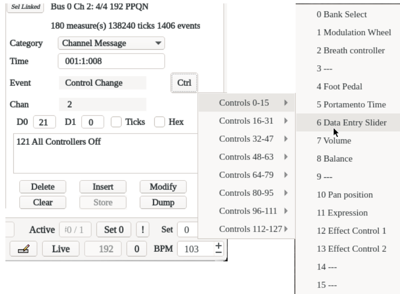
Figure 52: Control Change Button Drop-Down
