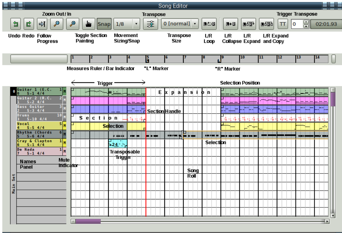
Figure 49: Song Editor Window, Annotated
