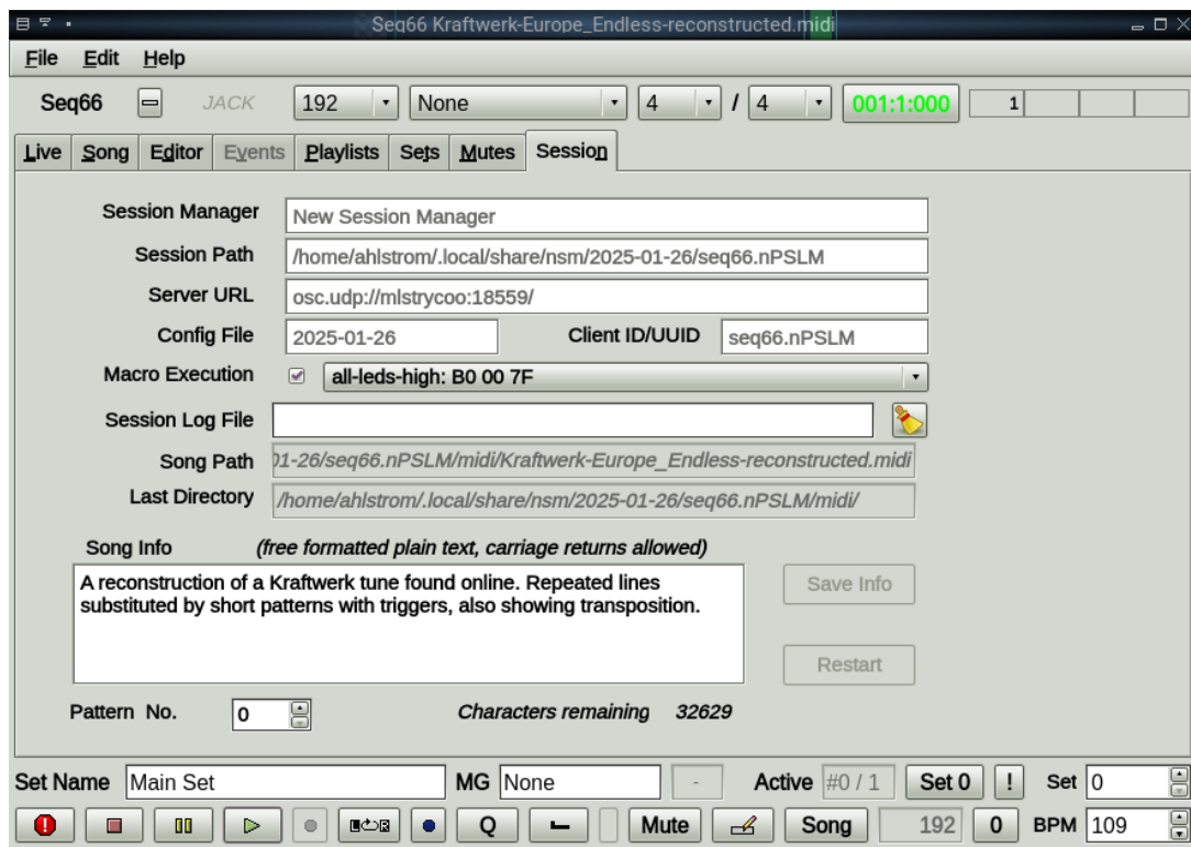
Session Tab with Song Info
