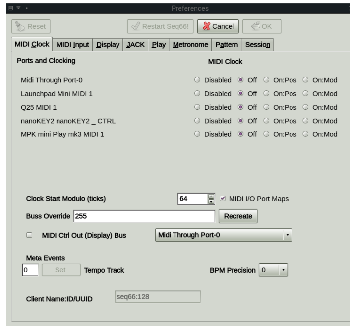
Figure 73: Clocks List With Port Mapping
