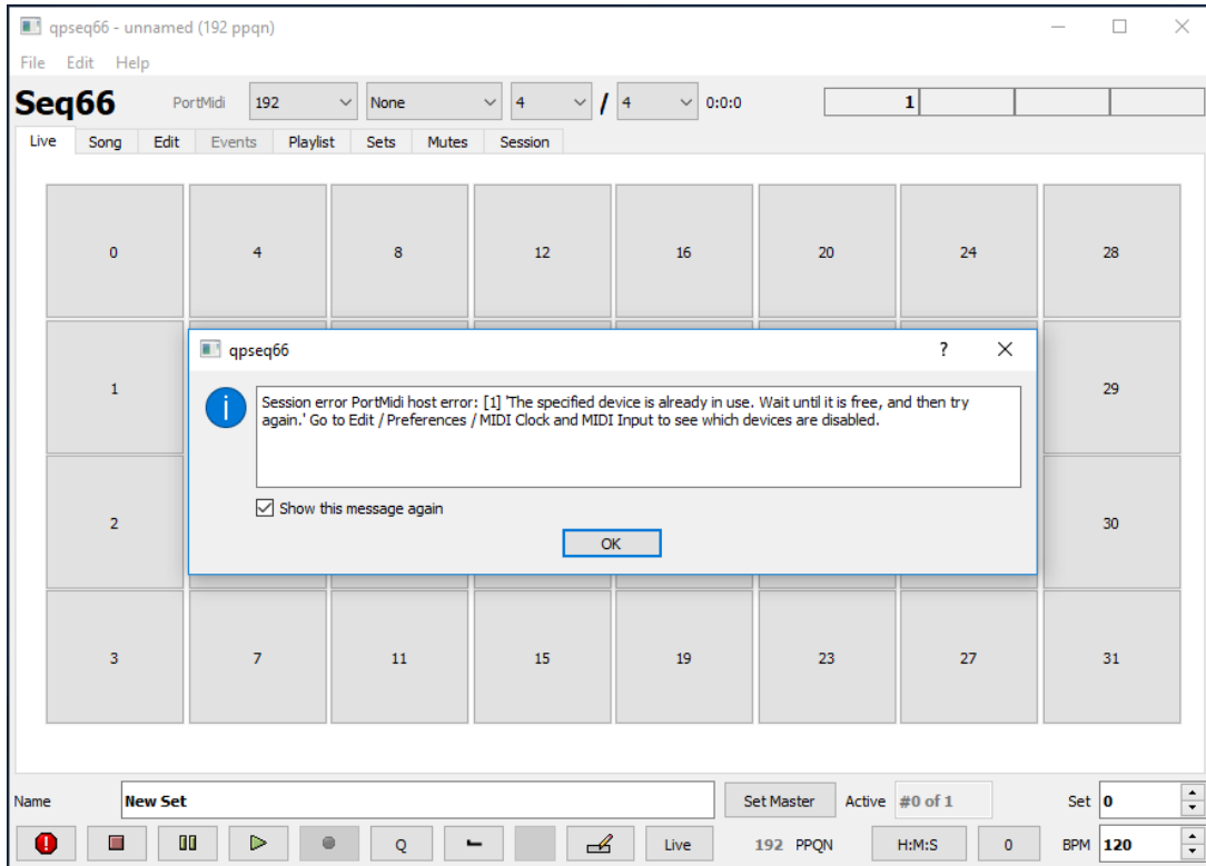
Figure 67: Seq66 First Startup in Windows
