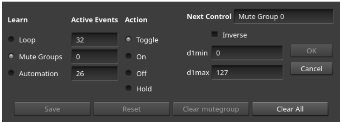
Figure 75: Seq66 Learn Manager
