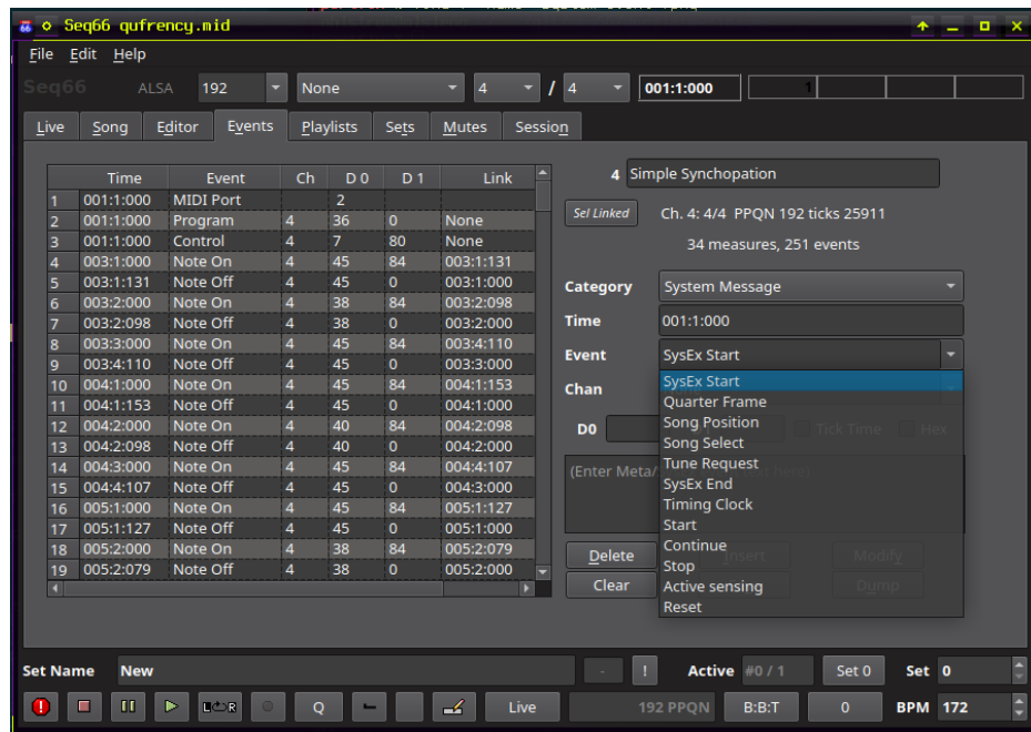
Figure 56: System Message List
