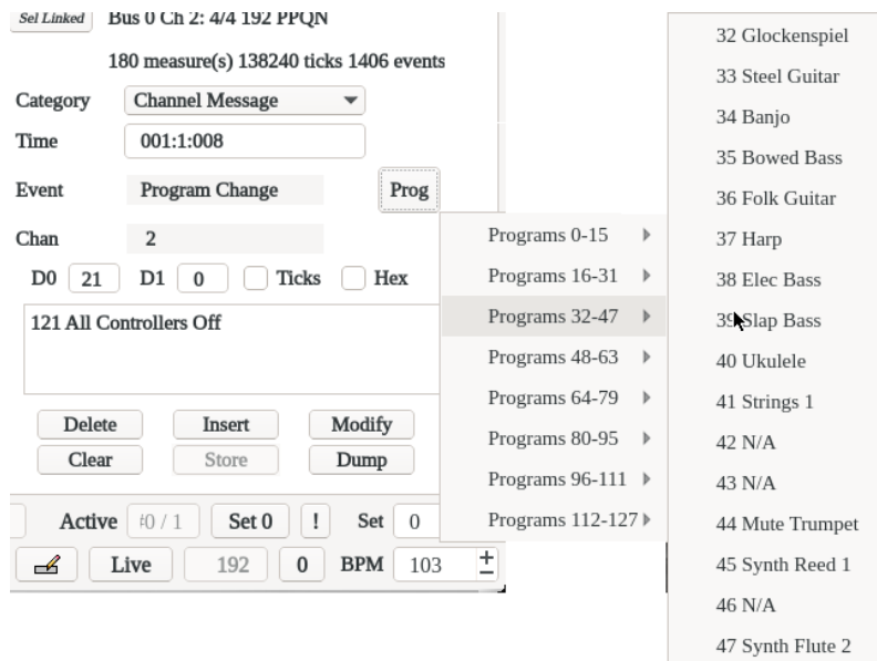
Figure 53: Program Change Button Drop-Down
