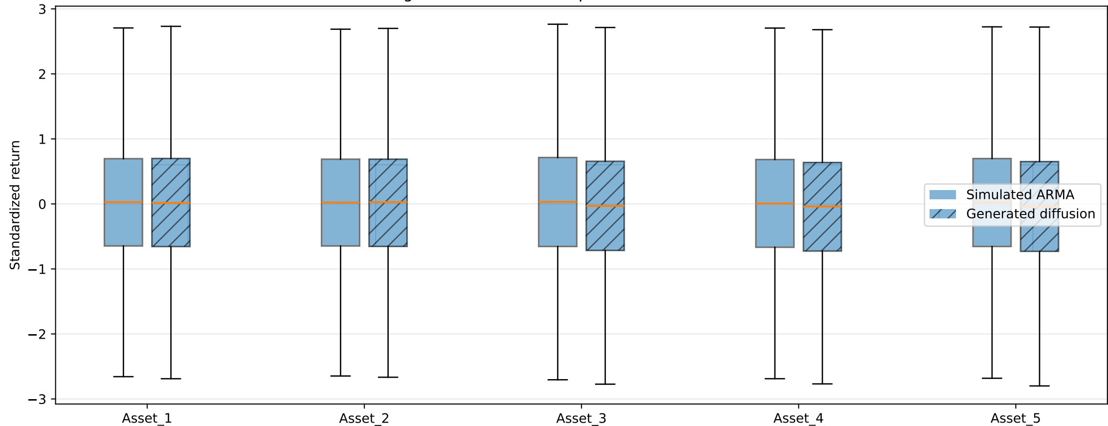
Marginal Distribution Comparison: ARMA vs Diffusion
