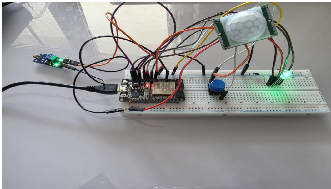
Green mode after pressing the button
