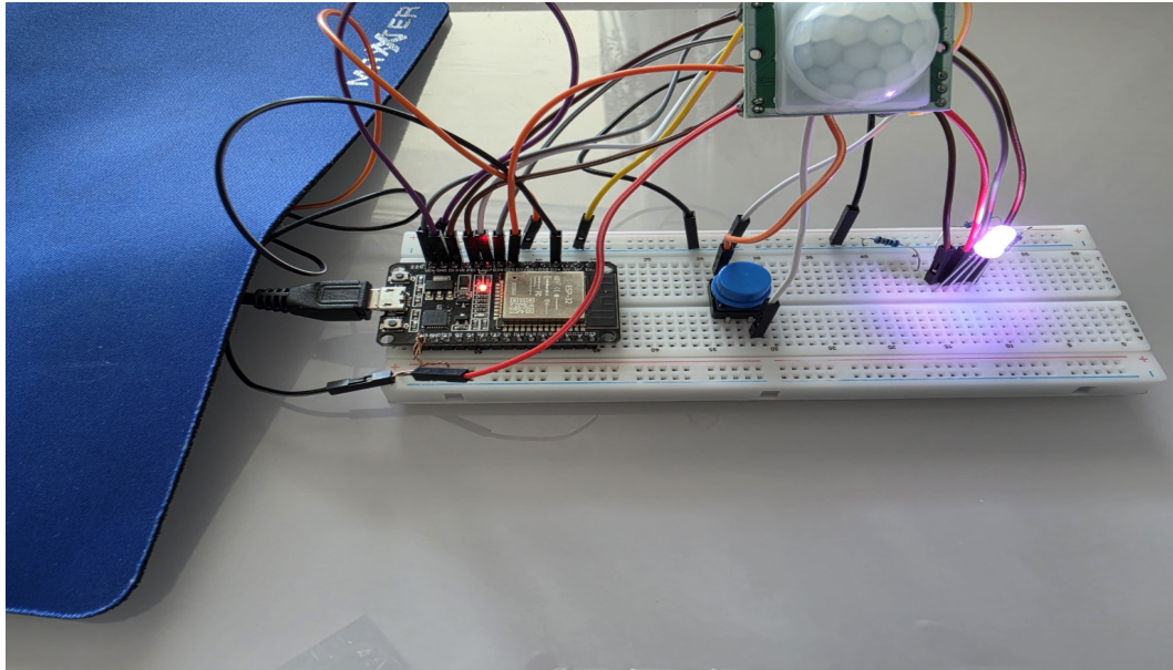
White light when motion is detected
