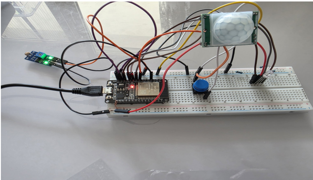
RGB light OFF because enough light is available
