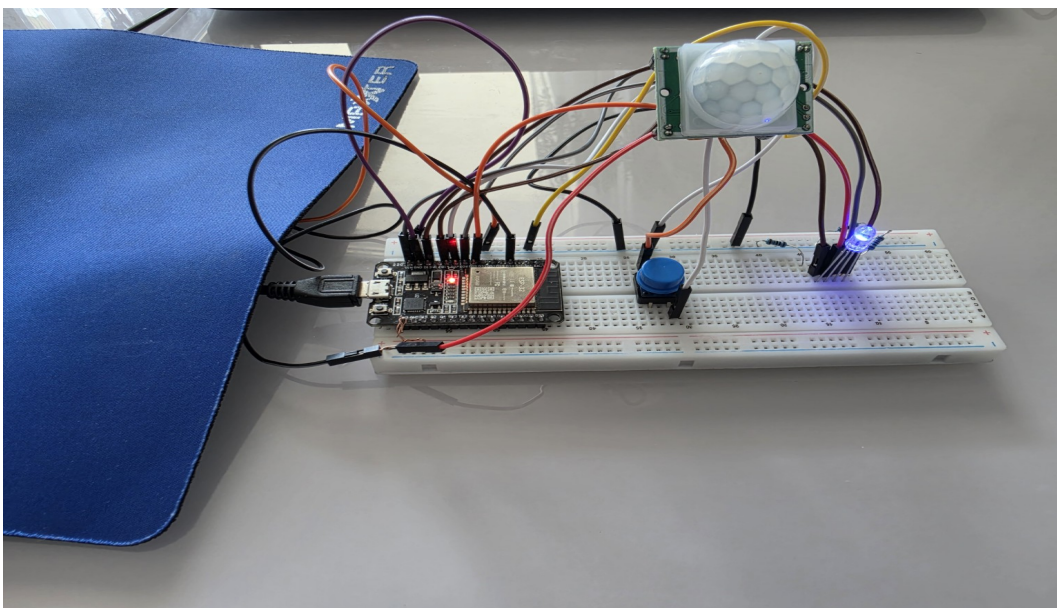
Blue standby light without motion
