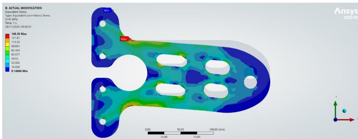
Figure 8: Modified Bracket Equivalent von-Mises Stress (MPa)
