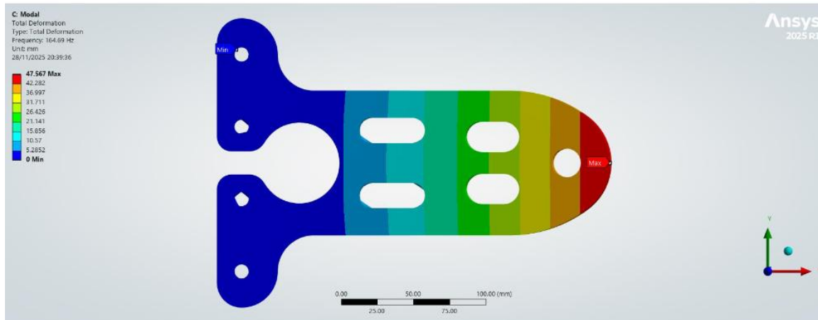
Figure 9: Modal Analysis of Modified Bracket (Mode 1)
