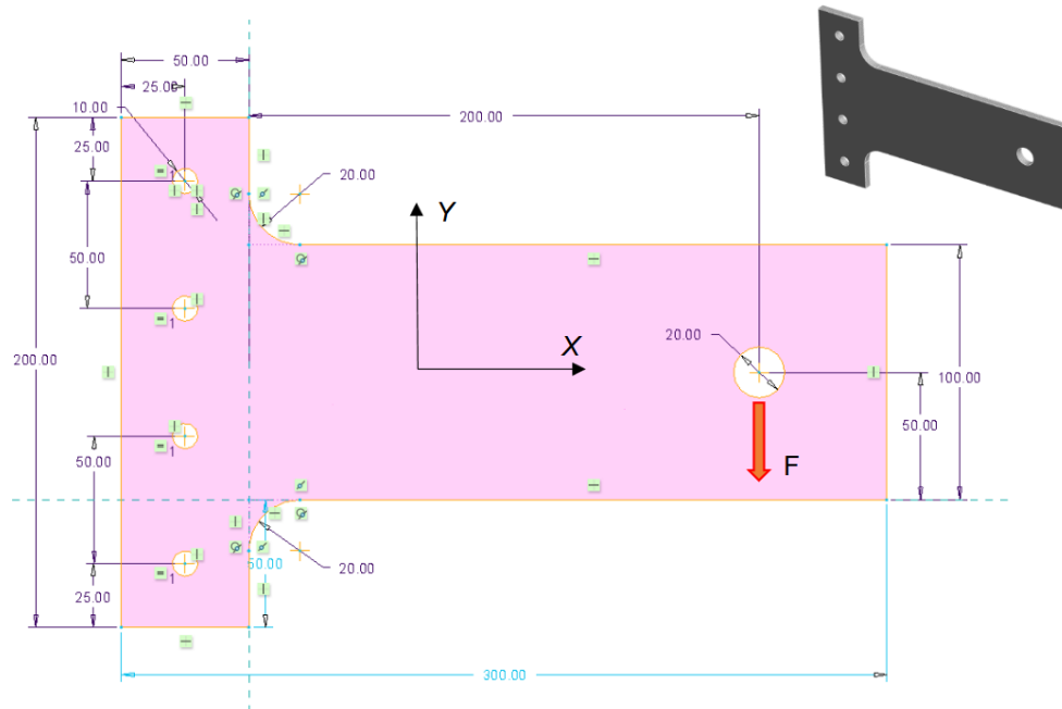
Figure 6: Original Bracket Geometry
