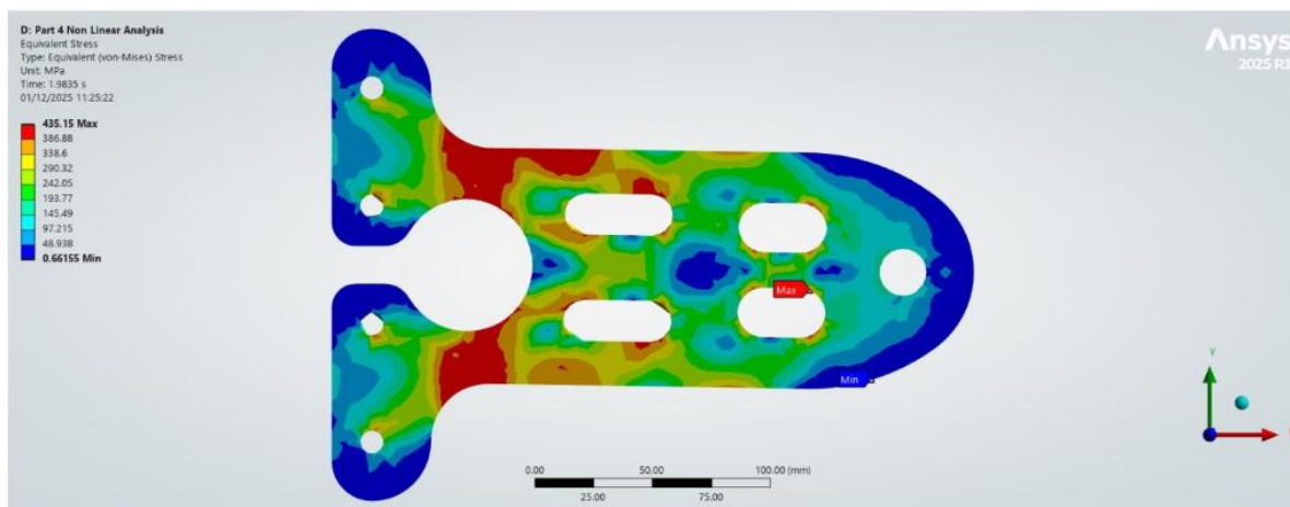
Figure 10: Modified Bracket Equivalent (von-Mises) Stress at Plastic Collapse Load
