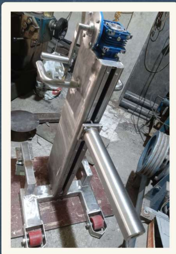
LIFTER ALUFOIL PENDEK
