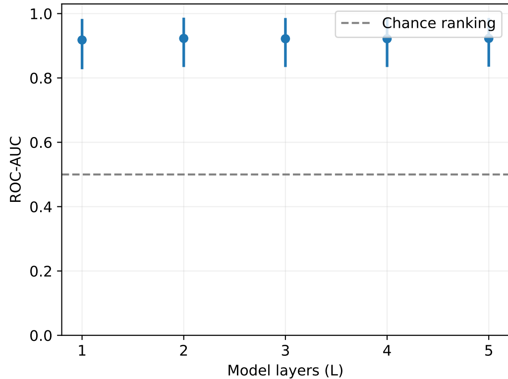
Ideal validation: 95% sample-bootstrap intervals
