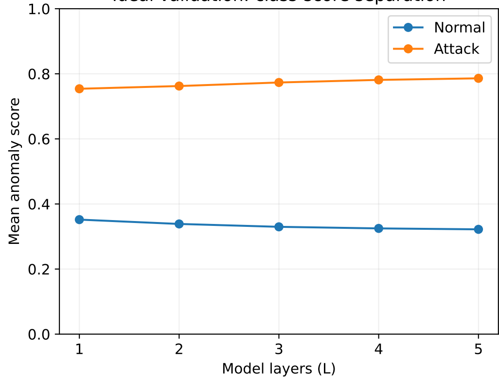
Ideal validation: class-score separation
