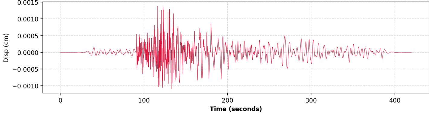
4. Displacement (HNZ | PGD: 0.001383 cm)
