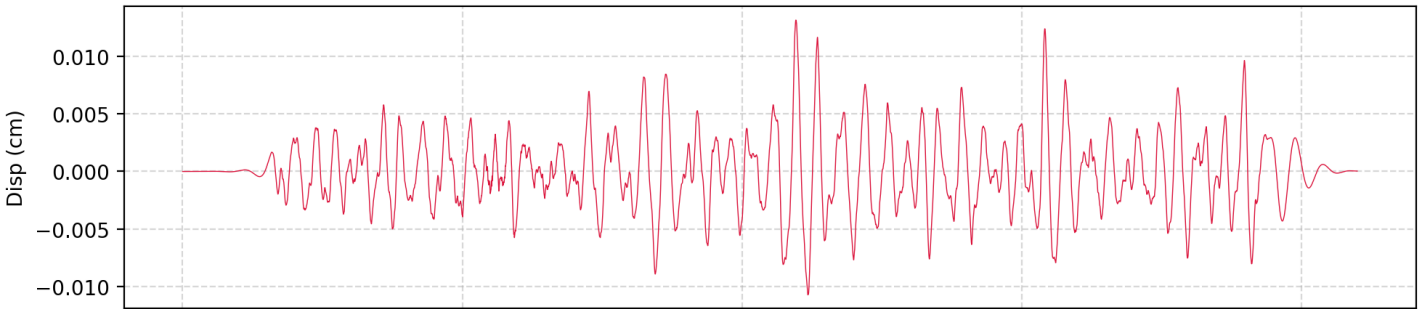
4. Displacement (HNE | PGD: 0.013126 cm)
