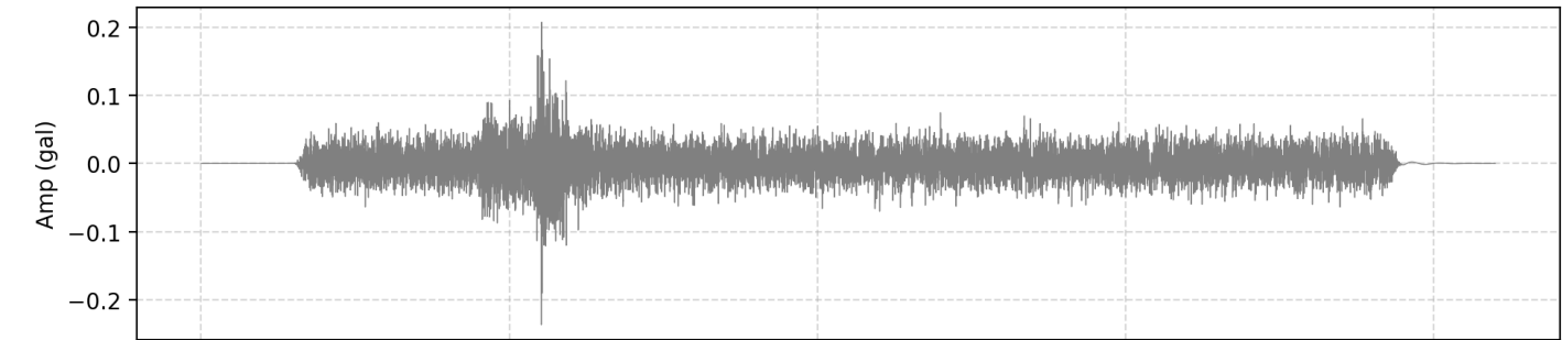
2. Filtered Acceleration (HNE | PGA: 0.002367 m/s 2 )
